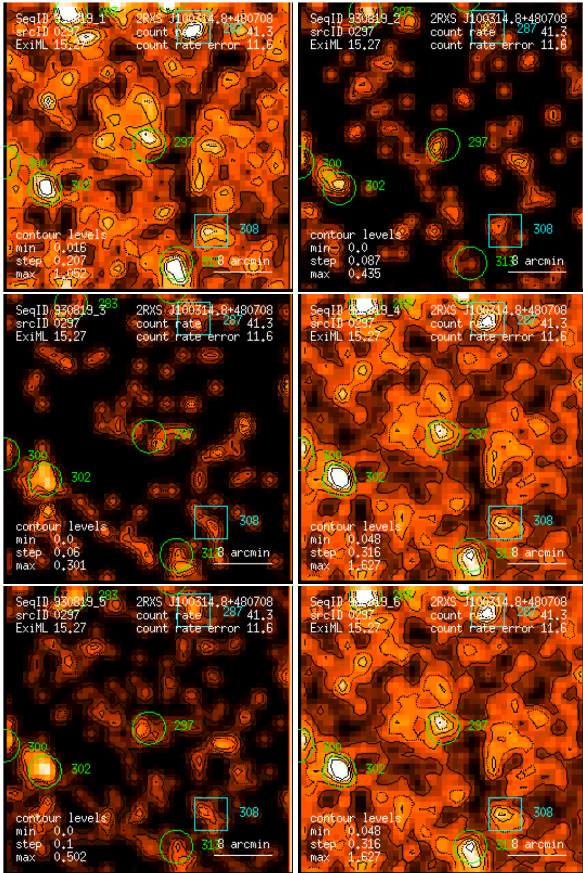
Figure 297: RASS 930819: detection 0297: band rate images, Gaussian filter: (1) PSPC channels 11 – 41, (2) 52 – 90, (3) 91 – 201, (4) 11 – 235, (5) 52 – 201, (6) 11 – 201. Broad band rates in counts/ks. Band rate contour levels in counts/ks/arcmin 2 .
