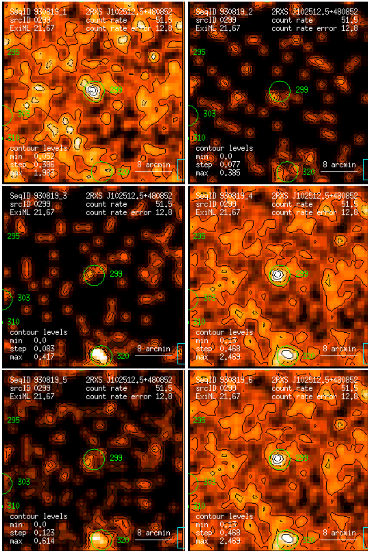
Figure 299: RASS 930819: detection 0299: band rate images, Gaussian filter: (1) PSPC channels 11 – 41, (2) 52 – 90, (3) 91 – 201, (4) 11 – 235, (5) 52 – 201, (6) 11 – 201. Broad band rates in counts/ks. Band rate contour levels in counts/ks/arcmin 2 .
