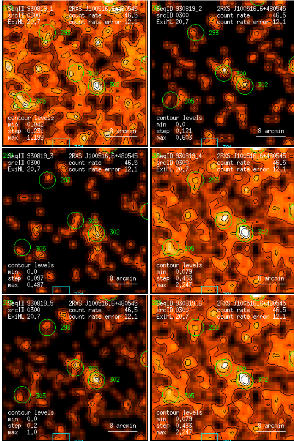
Figure 300: RASS 930819: detection 0300: band rate images, Gaussian filter: (1) PSPC channels 11 – 41, (2) 52 – 90, (3) 91 – 201, (4) 11 – 235, (5) 52 – 201, (6) 11 – 201. Broad band rates in counts/ks. Band rate contour levels in counts/ks/arcmin 2 .
