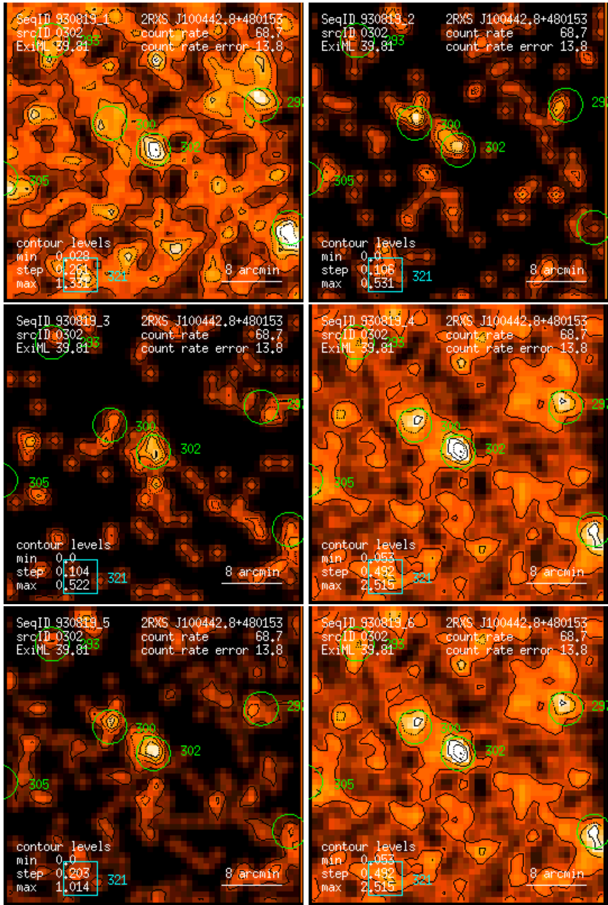
Figure 302: RASS 930819: detection 0302: band rate images, Gaussian filter: (1) PSPC channels 11 – 41, (2) 52 – 90, (3) 91 – 201, (4) 11 – 235, (5) 52 – 201, (6) 11 – 201. Broad band rates in counts/ks. Band rate contour levels in counts/ks/arcmin 2 .
