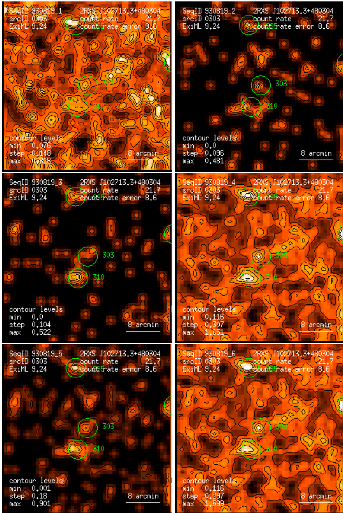
Figure 303: RASS 930819: detection 0303: band rate images, Gaussian filter: (1) PSPC channels 11 – 41, (2) 52 – 90, (3) 91 – 201, (4) 11 – 235, (5) 52 – 201, (6) 11 – 201. Broad band rates in counts/ks. Band rate contour levels in counts/ks/arcmin 2 .
