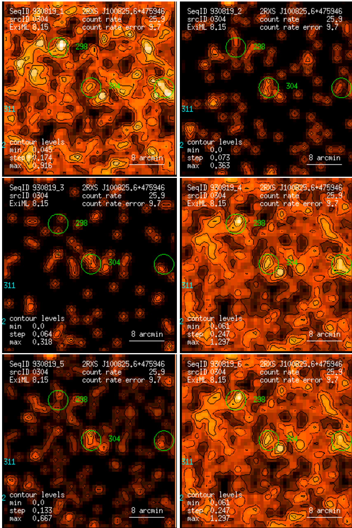
Figure 304: RASS 930819: detection 0304: band rate images, Gaussian filter: (1) PSPC channels 11 – 41, (2) 52 – 90, (3) 91 – 201, (4) 11 – 235, (5) 52 – 201, (6) 11 – 201. Broad band rates in counts/ks. Band rate contour levels in counts/ks/arcmin 2 .
