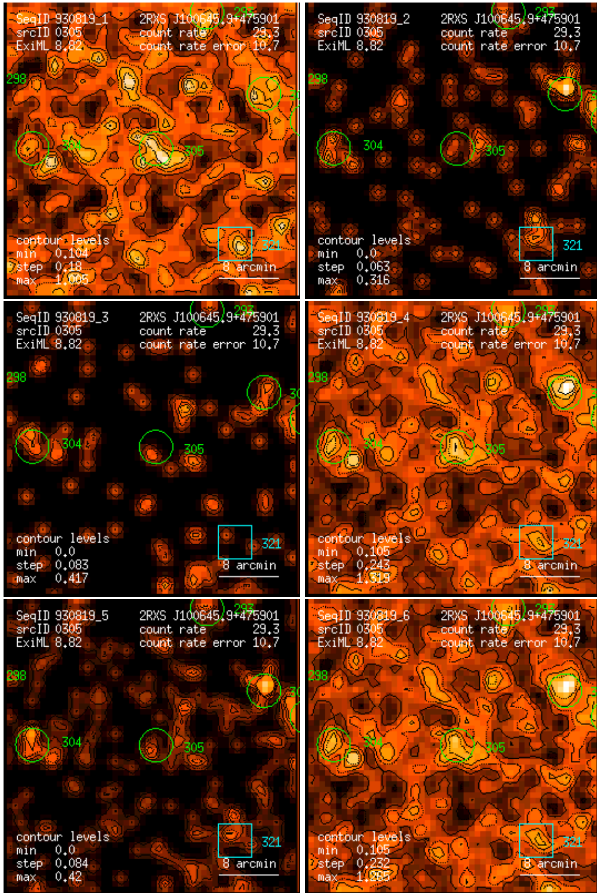
Figure 305: RASS 930819: detection 0305: band rate images, Gaussian filter: (1) PSPC channels 11 – 41, (2) 52 – 90, (3) 91 – 201, (4) 11 – 235, (5) 52 – 201, (6) 11 – 201. Broad band rates in counts/ks. Band rate contour levels in counts/ks/arcmin 2 .
