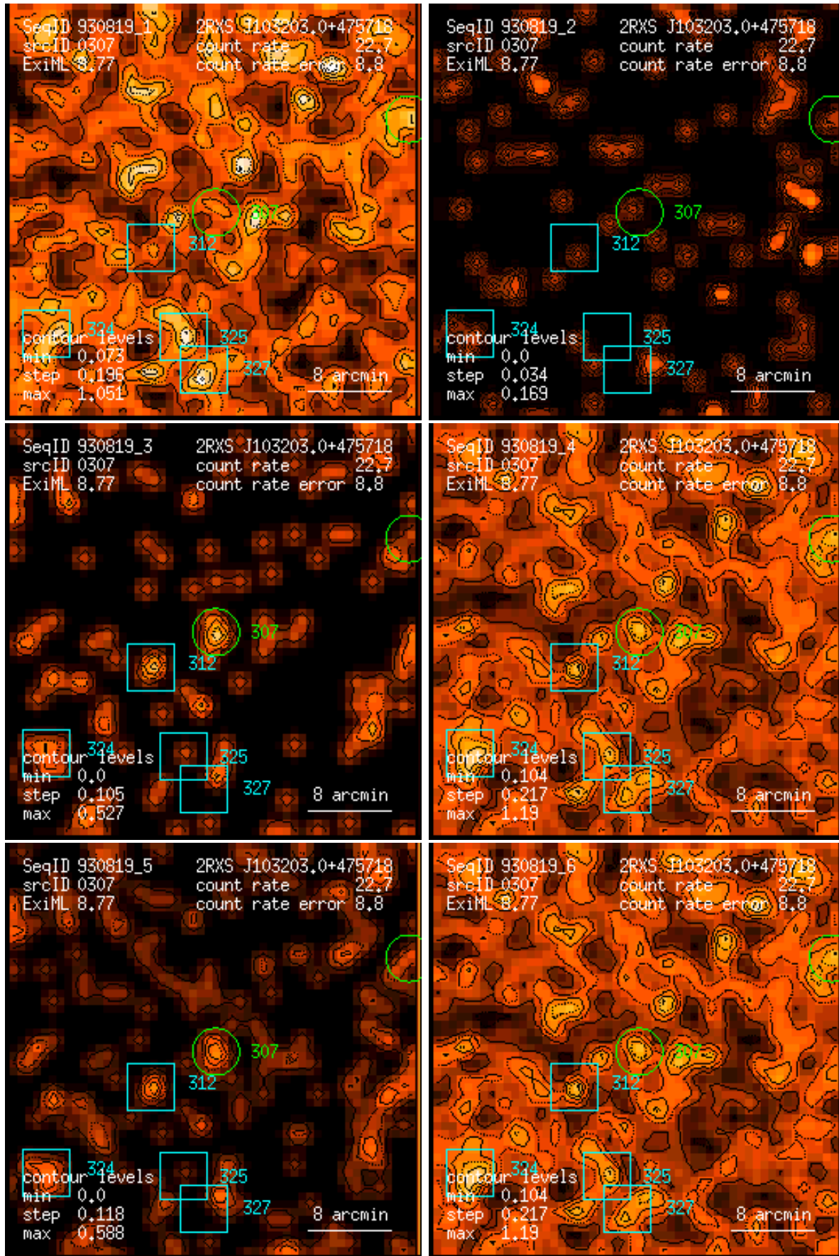
Figure 307: RASS 930819: detection 0307: band rate images, Gaussian filter: (1) PSPC channels 11 – 41, (2) 52 – 90, (3) 91 – 201, (4) 11 – 235, (5) 52 – 201, (6) 11 – 201. Broad band rates in counts/ks. Band rate contour levels in counts/ks/arcmin 2 .
