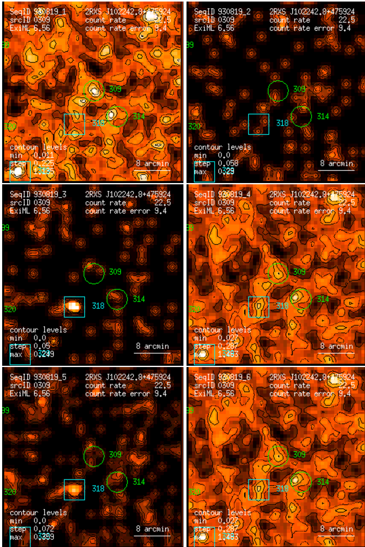
Figure 309: RASS 930819: detection 0309: band rate images, Gaussian filter: (1) PSPC channels 11 – 41, (2) 52 – 90, (3) 91 – 201, (4) 11 – 235, (5) 52 – 201, (6) 11 – 201. Broad band rates in counts/ks. Band rate contour levels in counts/ks/arcmin 2 .
