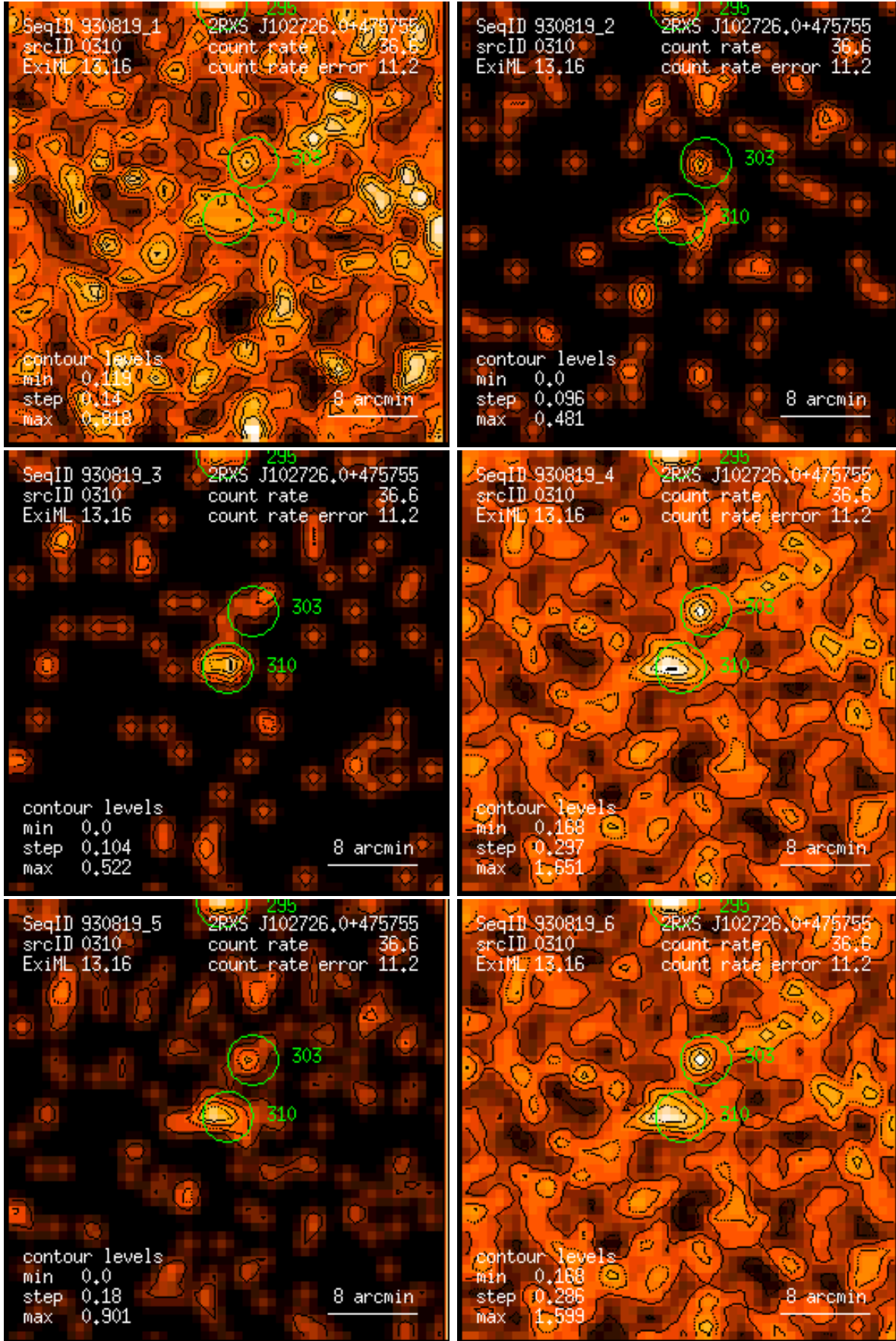
Figure 310: RASS 930819: detection 0310: band rate images, Gaussian filter: (1) PSPC channels 11 – 41, (2) 52 – 90, (3) 91 – 201, (4) 11 – 235, (5) 52 – 201, (6) 11 – 201. Broad band rates in counts/ks. Band rate contour levels in counts/ks/arcmin 2 .
