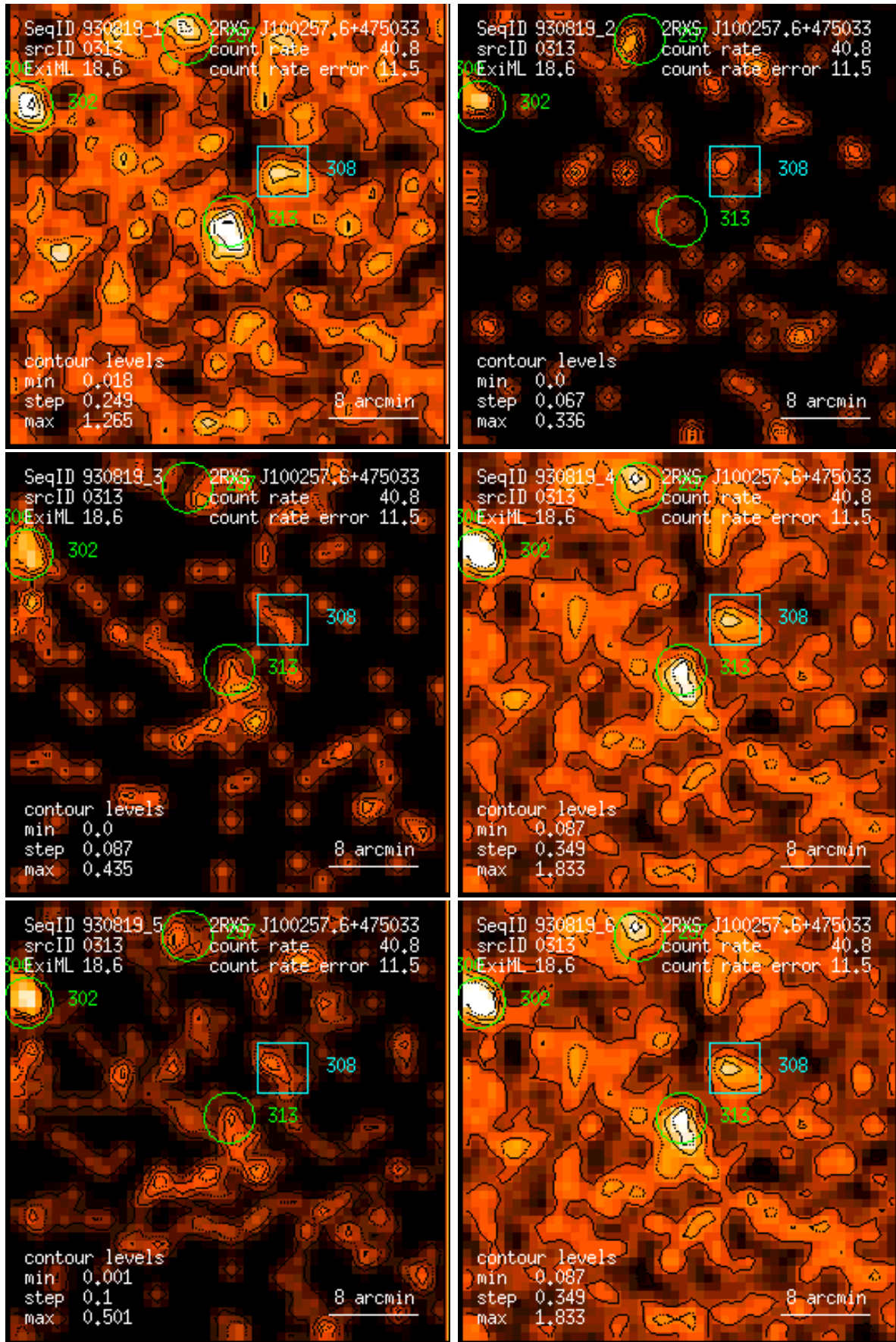
Figure 313: RASS 930819: detection 0313: band rate images, Gaussian filter: (1) PSPC channels 11 – 41, (2) 52 – 90, (3) 91 – 201, (4) 11 – 235, (5) 52 – 201, (6) 11 – 201. Broad band rates in counts/ks. Band rate contour levels in counts/ks/arcmin 2 .
