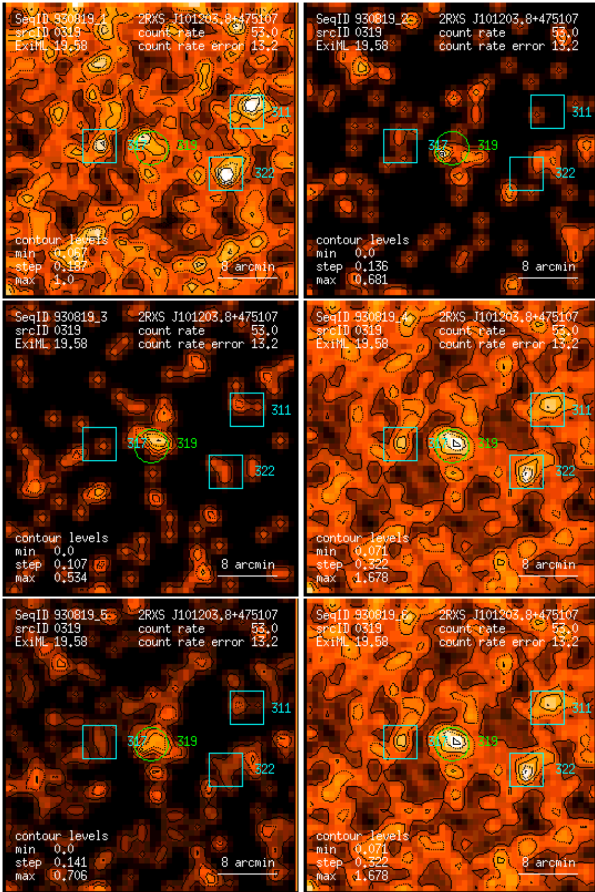
Figure 319: RASS 930819: detection 0319: band rate images, Gaussian filter: (1) PSPC channels 11 – 41, (2) 52 – 90, (3) 91 – 201, (4) 11 – 235, (5) 52 – 201, (6) 11 – 201. Broad band rates in counts/ks. Band rate contour levels in counts/ks/arcmin 2 .
