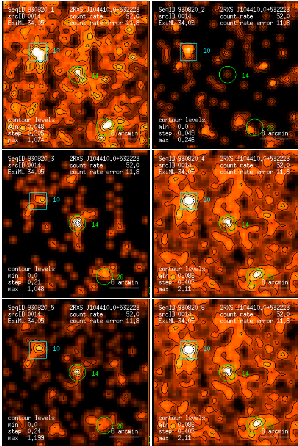
Figure 14: RASS 930820: detection 0014: band rate images, Gaussian filter: (1) PSPC channels 11 – 41, (2) 52 – 90, (3) 91 – 201, (4) 11 – 235, (5) 52 – 201, (6) 11 – 201. Broad band rates in counts/ks. Band rate contour levels in counts/ks/arcmin 2 .
