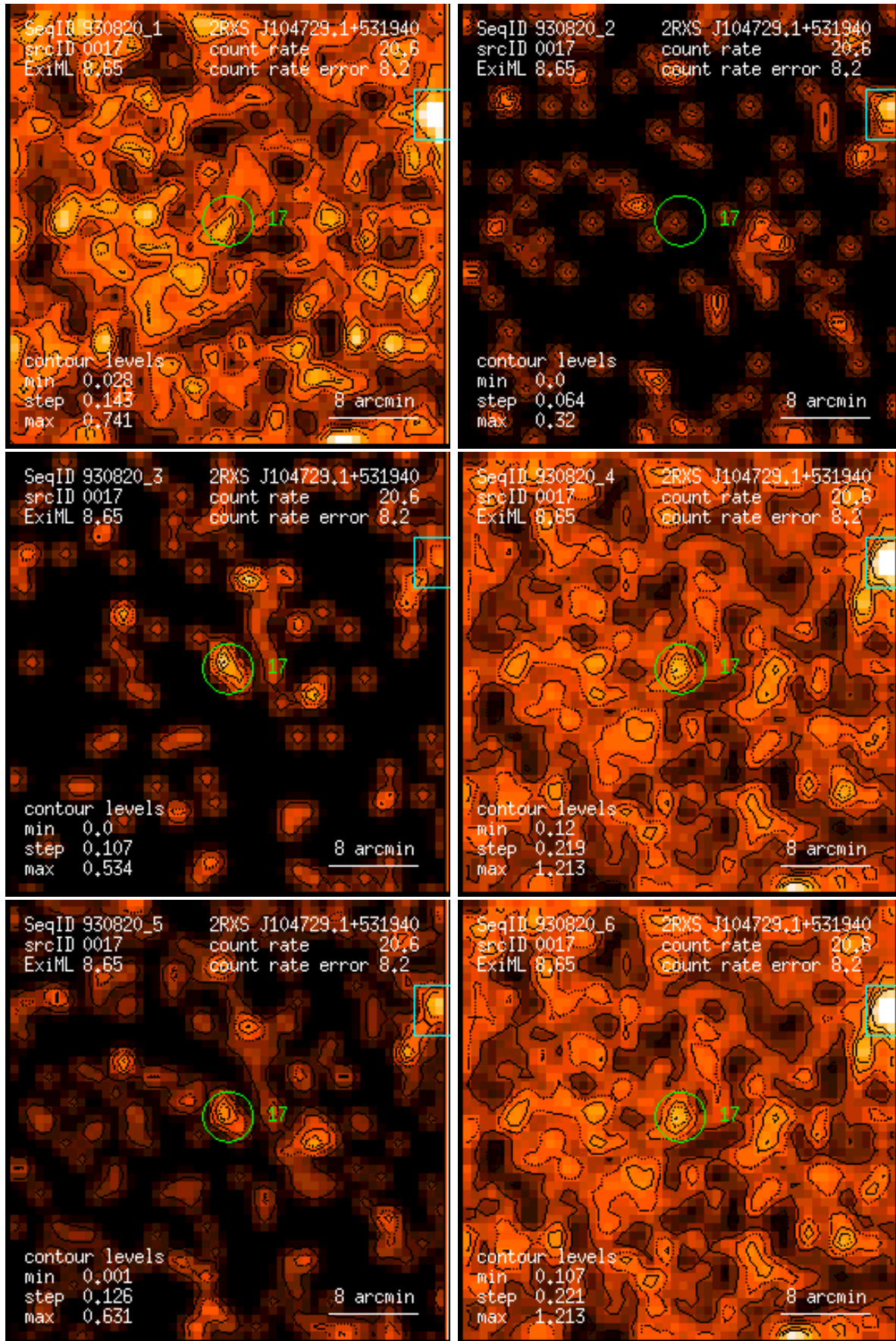
Figure 17: RASS 930820: detection 0017: band rate images, Gaussian filter: (1) PSPC channels 11 – 41, (2) 52 – 90, (3) 91 – 201, (4) 11 – 235, (5) 52 – 201, (6) 11 – 201. Broad band rates in counts/ks. Band rate contour levels in counts/ks/arcmin 2 .
