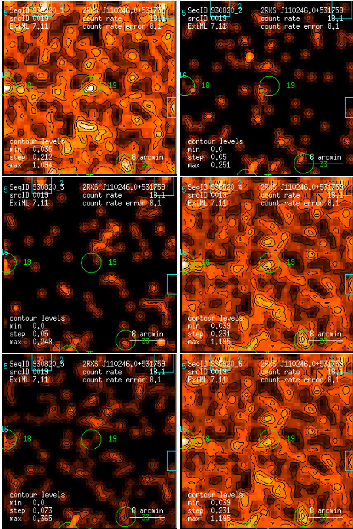
Figure 19: RASS 930820: detection 0019: band rate images, Gaussian filter: (1) PSPC channels 11 – 41, (2) 52 – 90, (3) 91 – 201, (4) 11 – 235, (5) 52 – 201, (6) 11 – 201. Broad band rates in counts/ks. Band rate contour levels in counts/ks/arcmin 2 .
