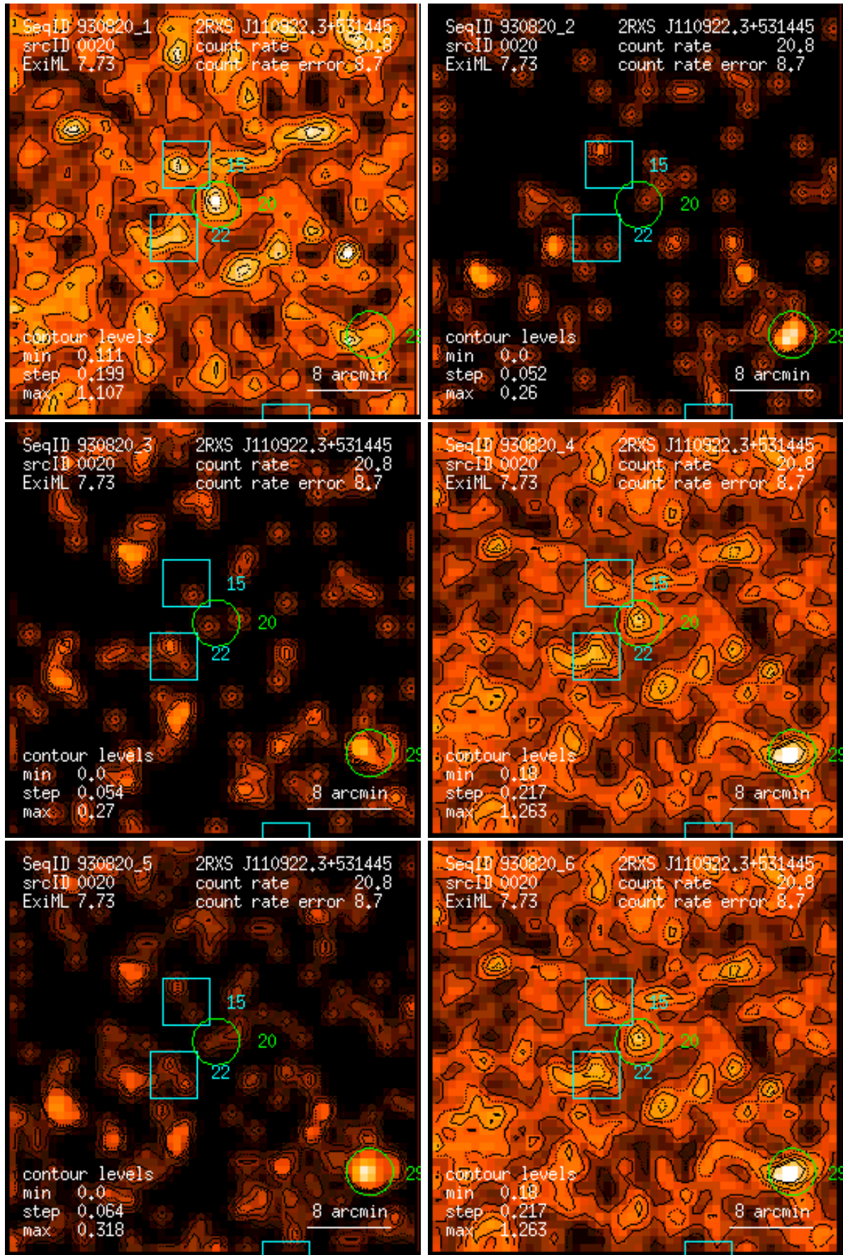
Figure 20: RASS 930820: detection 0020: band rate images, Gaussian filter: (1) PSPC channels 11 – 41, (2) 52 – 90, (3) 91 – 201, (4) 11 – 235, (5) 52 – 201, (6) 11 – 201. Broad band rates in counts/ks. Band rate contour levels in counts/ks/arcmin 2 .
