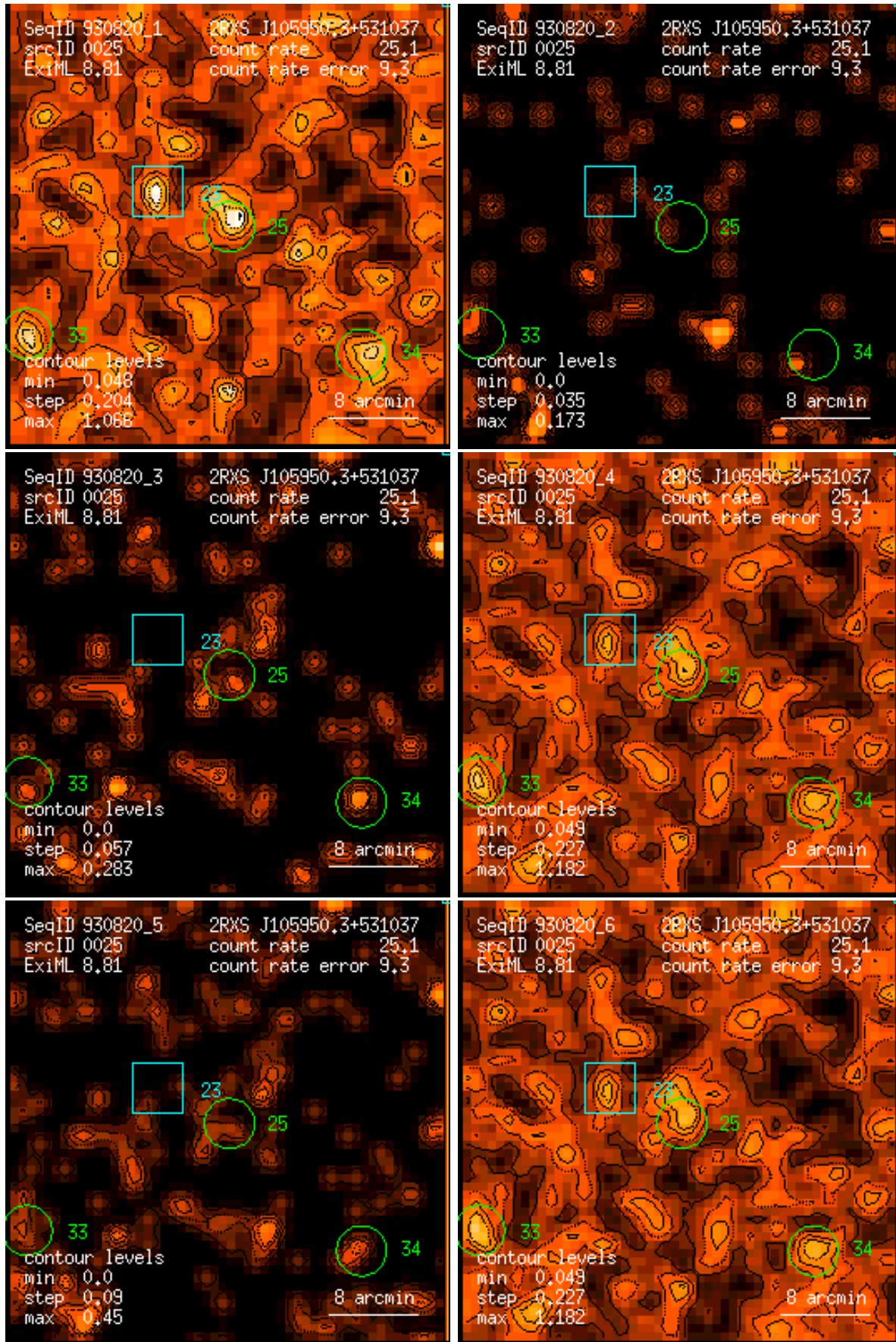
Figure 25: RASS 930820: detection 0025: band rate images, Gaussian filter: (1) PSPC channels 11 – 41, (2) 52 – 90, (3) 91 – 201, (4) 11 – 235, (5) 52 – 201, (6) 11 – 201. Broad band rates in counts/ks. Band rate contour levels in counts/ks/arcmin 2 .
