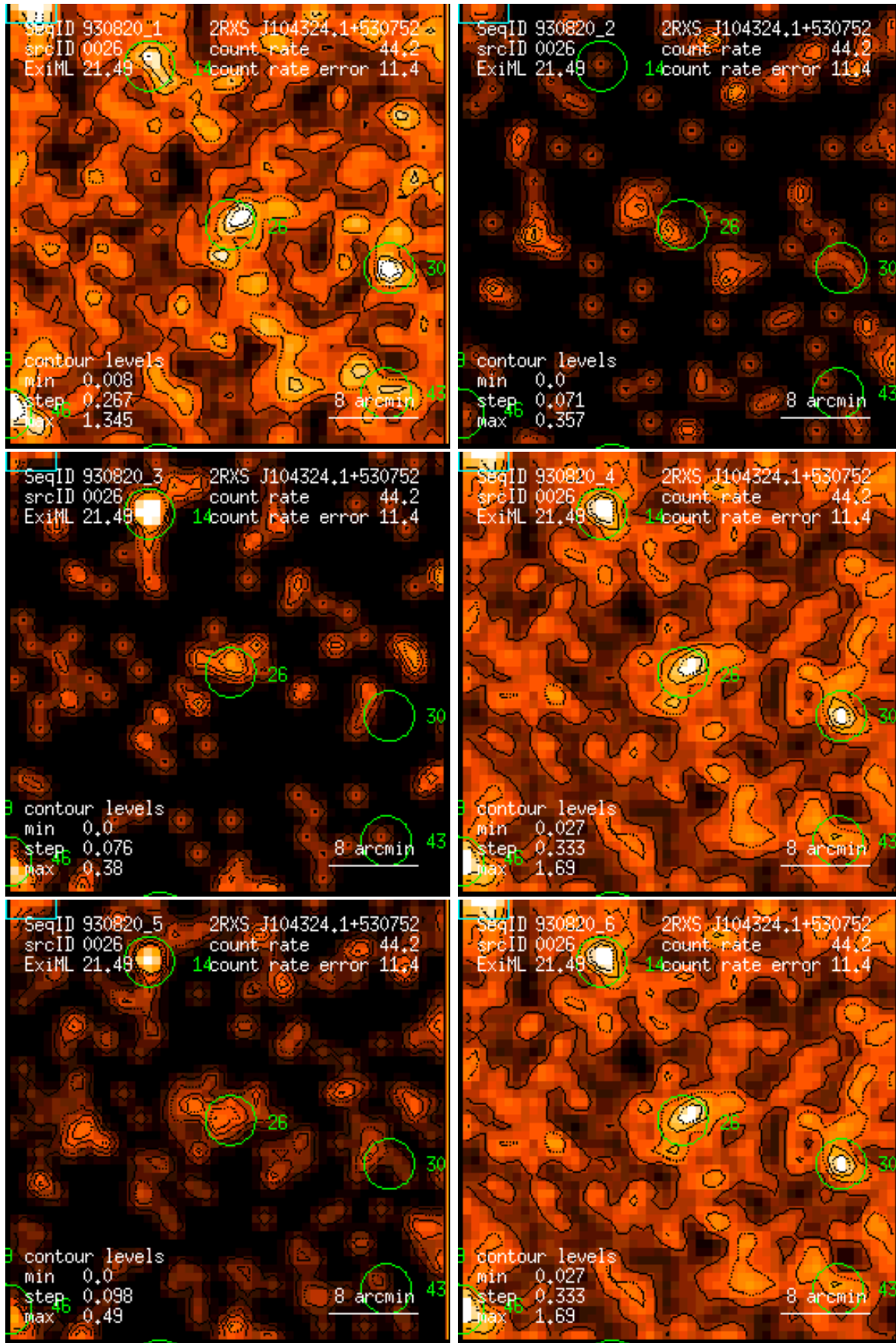
Figure 26: RASS 930820: detection 0026: band rate images, Gaussian filter: (1) PSPC channels 11 – 41, (2) 52 – 90, (3) 91 – 201, (4) 11 – 235, (5) 52 – 201, (6) 11 – 201. Broad band rates in counts/ks. Band rate contour levels in counts/ks/arcmin 2 .
