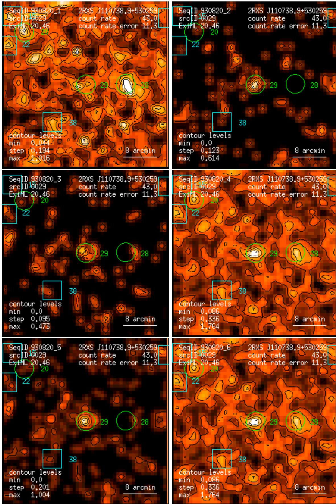
Figure 29: RASS 930820: detection 0029: band rate images, Gaussian filter: (1) PSPC channels 11 – 41, (2) 52 – 90, (3) 91 – 201, (4) 11 – 235, (5) 52 – 201, (6) 11 – 201. Broad band rates in counts/ks. Band rate contour levels in counts/ks/arcmin 2 .
