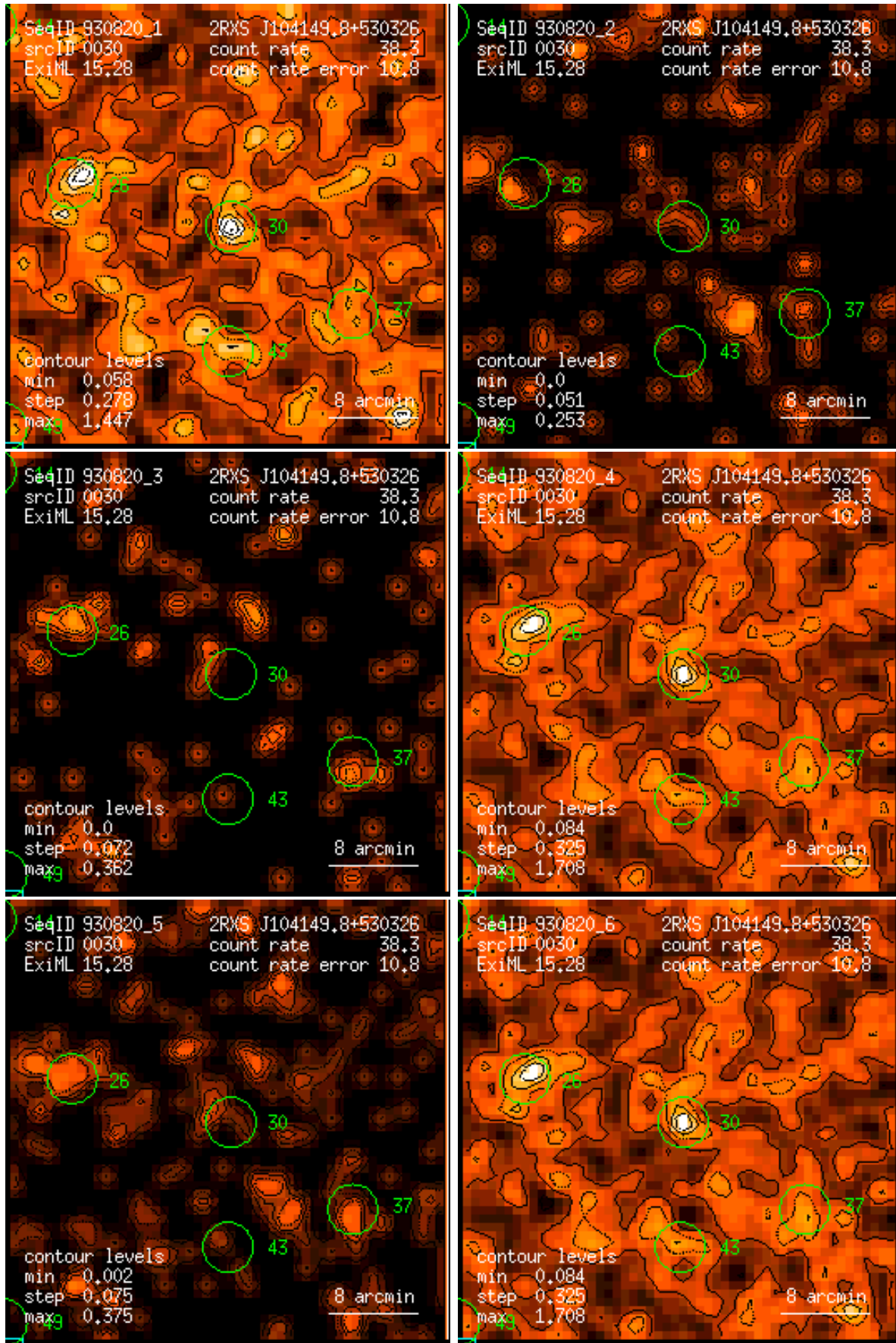
Figure 30: RASS 930820: detection 0030: band rate images, Gaussian filter: (1) PSPC channels 11 – 41, (2) 52 – 90, (3) 91 – 201, (4) 11 – 235, (5) 52 – 201, (6) 11 – 201. Broad band rates in counts/ks. Band rate contour levels in counts/ks/arcmin 2 .
