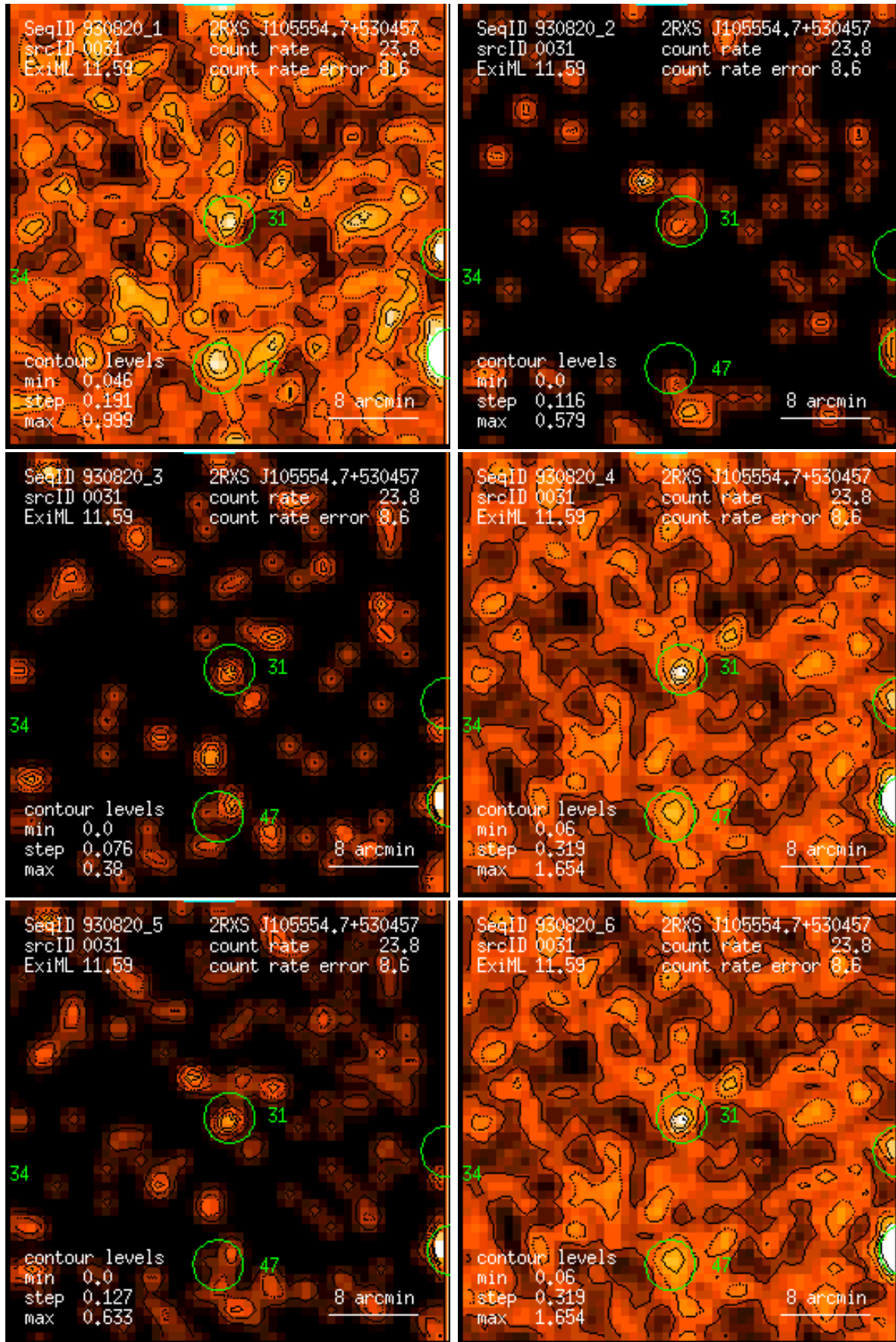
Figure 31: RASS 930820: detection 0031: band rate images, Gaussian filter: (1) PSPC channels 11 – 41, (2) 52 – 90, (3) 91 – 201, (4) 11 – 235, (5) 52 – 201, (6) 11 – 201. Broad band rates in counts/ks. Band rate contour levels in counts/ks/arcmin 2 .
