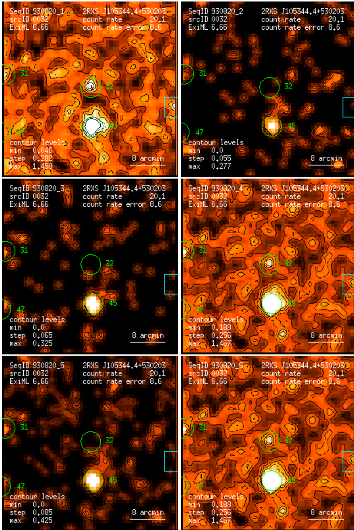
Figure 32: RASS 930820: detection 0032: band rate images, Gaussian filter: (1) PSPC channels 11 – 41, (2) 52 – 90, (3) 91 – 201, (4) 11 – 235, (5) 52 – 201, (6) 11 – 201. Broad band rates in counts/ks. Band rate contour levels in counts/ks/arcmin 2 .
