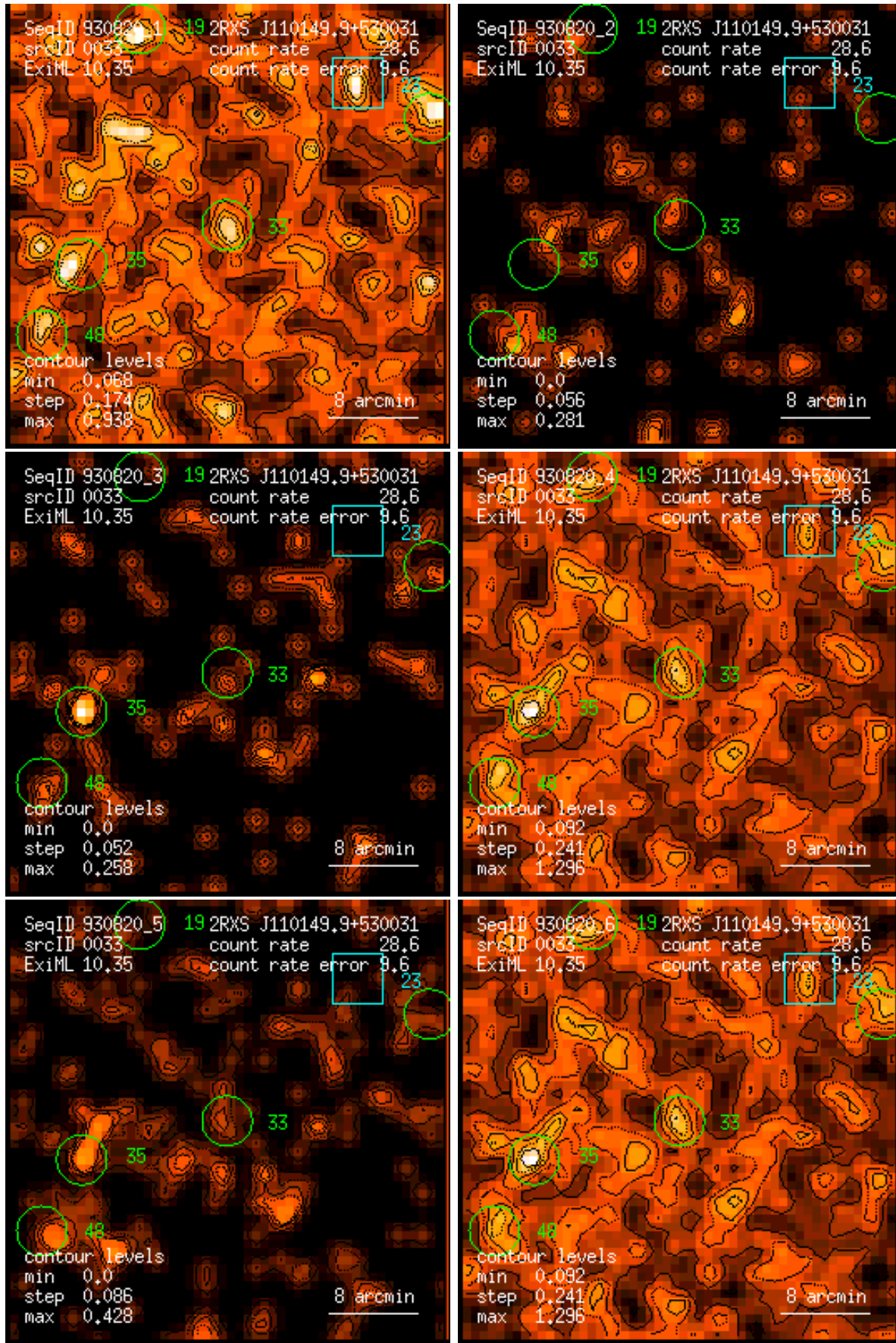
Figure 33: RASS 930820: detection 0033: band rate images, Gaussian filter: (1) PSPC channels 11 – 41, (2) 52 – 90, (3) 91 – 201, (4) 11 – 235, (5) 52 – 201, (6) 11 – 201. Broad band rates in counts/ks. Band rate contour levels in counts/ks/arcmin 2 .
