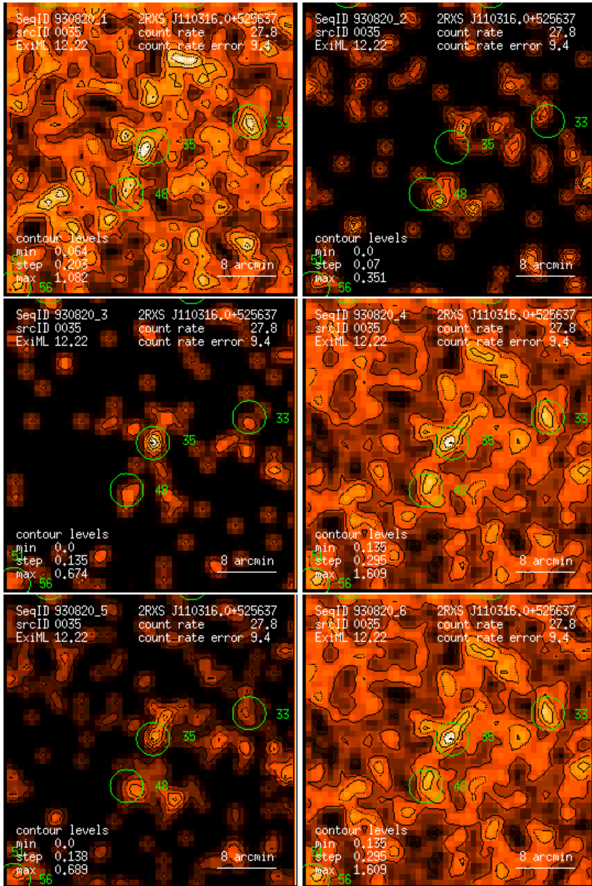
Figure 35: RASS 930820: detection 0035: band rate images, Gaussian filter: (1) PSPC channels 11 – 41, (2) 52 – 90, (3) 91 – 201, (4) 11 – 235, (5) 52 – 201, (6) 11 – 201. Broad band rates in counts/ks. Band rate contour levels in counts/ks/arcmin 2 .
