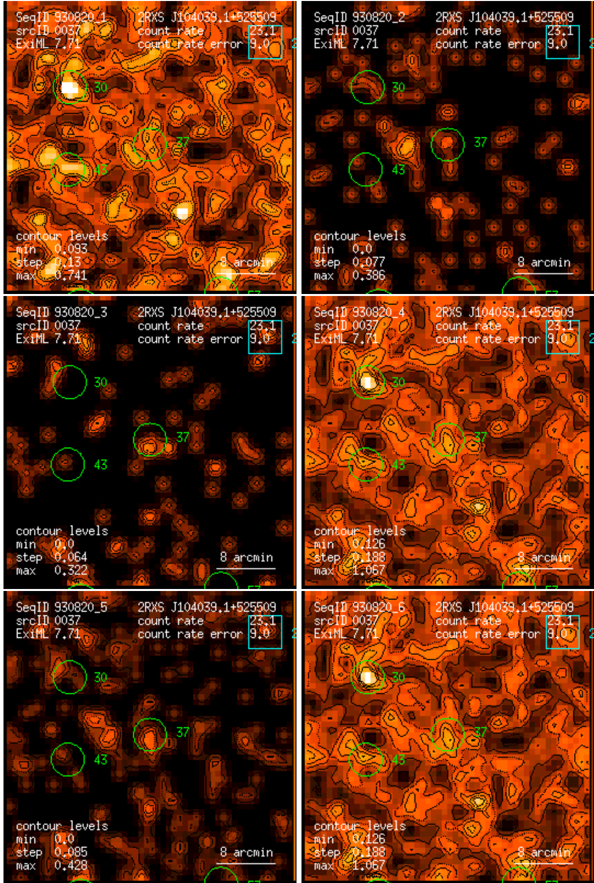
Figure 37: RASS 930820: detection 0037: band rate images, Gaussian filter: (1) PSPC channels 11 – 41, (2) 52 – 90, (3) 91 – 201, (4) 11 – 235, (5) 52 – 201, (6) 11 – 201. Broad band rates in counts/ks. Band rate contour levels in counts/ks/arcmin 2 .
