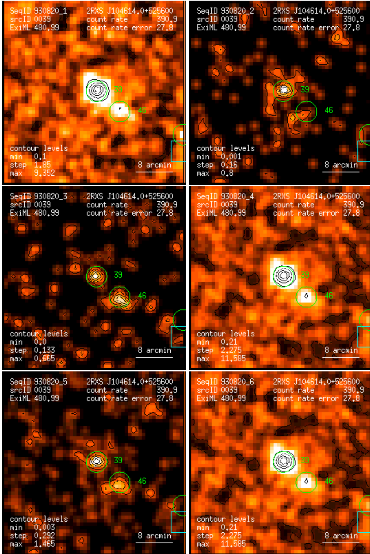
Figure 39: RASS 930820: detection 0039: band rate images, Gaussian filter: (1) PSPC channels 11 – 41, (2) 52 – 90, (3) 91 – 201, (4) 11 – 235, (5) 52 – 201, (6) 11 – 201. Broad band rates in counts/ks. Band rate contour levels in counts/ks/arcmin 2 .
