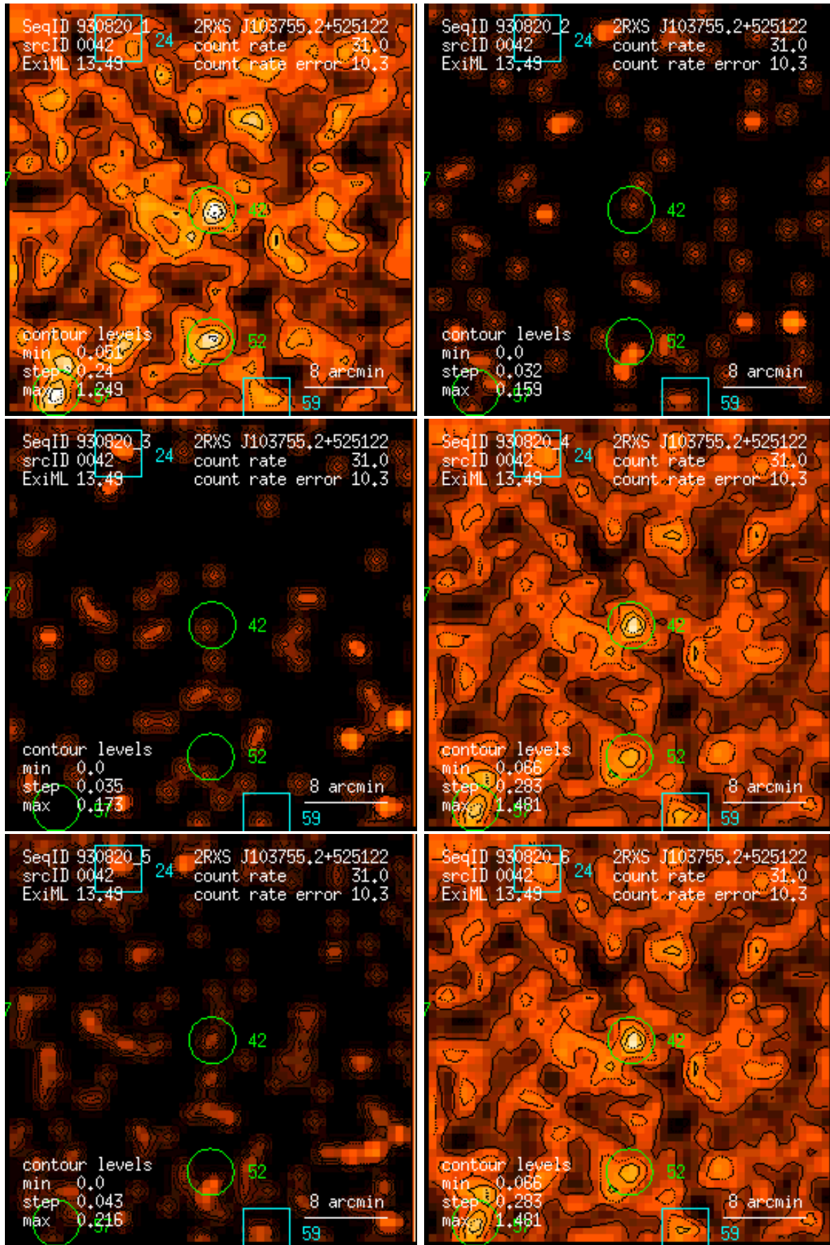
Figure 42: RASS 930820: detection 0042: band rate images, Gaussian filter: (1) PSPC channels 11 – 41, (2) 52 – 90, (3) 91 – 201, (4) 11 – 235, (5) 52 – 201, (6) 11 – 201. Broad band rates in counts/ks. Band rate contour levels in counts/ks/arcmin 2 .
