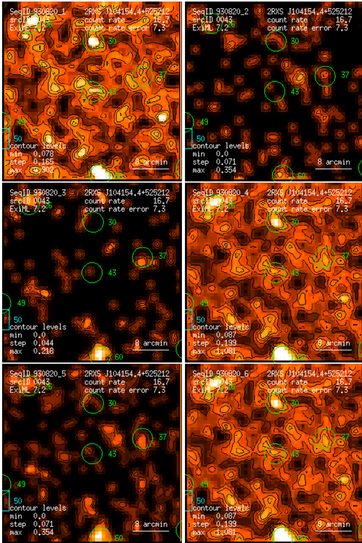
Figure 43: RASS 930820: detection 0043: band rate images, Gaussian filter: (1) PSPC channels 11 – 41, (2) 52 – 90, (3) 91 – 201, (4) 11 – 235, (5) 52 – 201, (6) 11 – 201. Broad band rates in counts/ks. Band rate contour levels in counts/ks/arcmin 2 .
