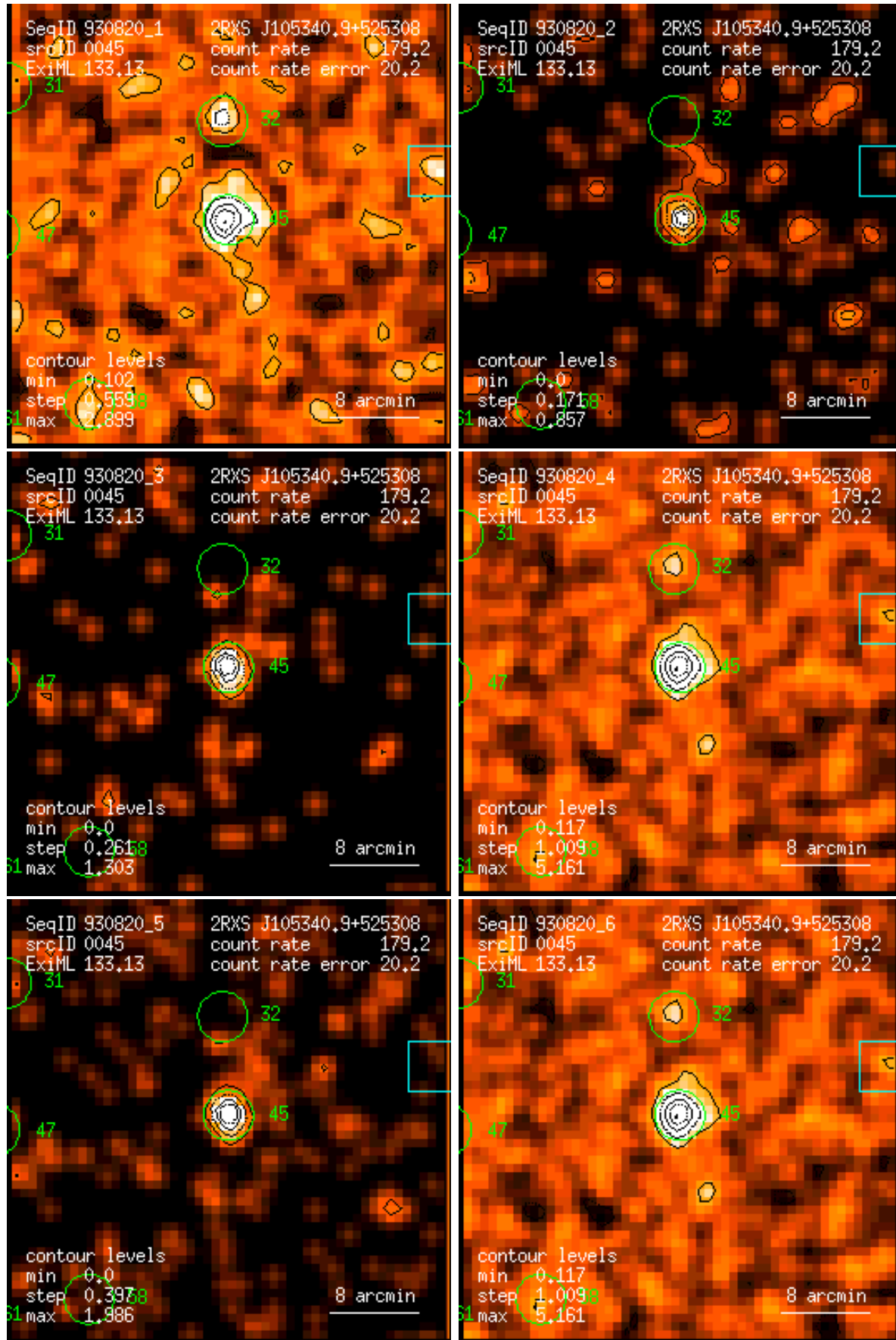
Figure 45: RASS 930820: detection 0045: band rate images, Gaussian filter: (1) PSPC channels 11 – 41, (2) 52 – 90, (3) 91 – 201, (4) 11 – 235, (5) 52 – 201, (6) 11 – 201. Broad band rates in counts/ks. Band rate contour levels in counts/ks/arcmin 2 .
