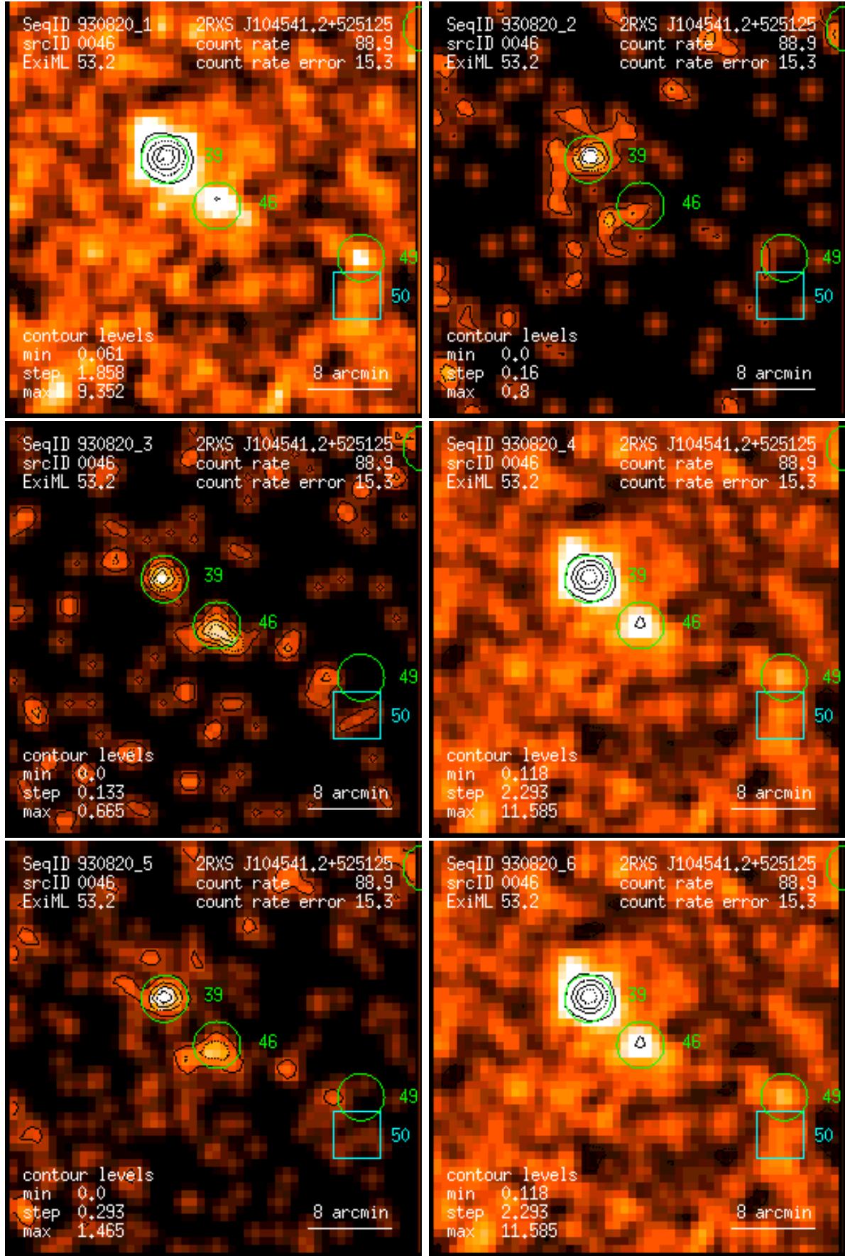
Figure 46: RASS 930820: detection 0046: band rate images, Gaussian filter: (1) PSPC channels 11 – 41, (2) 52 – 90, (3) 91 – 201, (4) 11 – 235, (5) 52 – 201, (6) 11 – 201. Broad band rates in counts/ks. Band rate contour levels in counts/ks/arcmin 2 .
