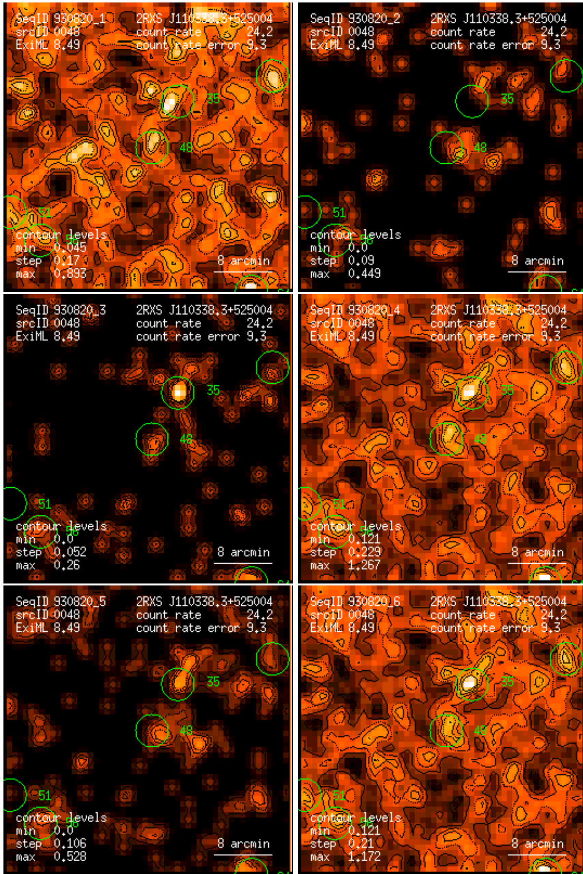
Figure 48: RASS 930820: detection 0048: band rate images, Gaussian filter: (1) PSPC channels 11 – 41, (2) 52 – 90, (3) 91 – 201, (4) 11 – 235, (5) 52 – 201, (6) 11 – 201. Broad band rates in counts/ks. Band rate contour levels in counts/ks/arcmin 2 .
