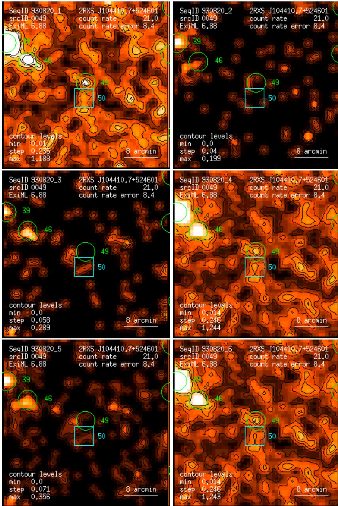
Figure 49: RASS 930820: detection 0049: band rate images, Gaussian filter: (1) PSPC channels 11 – 41, (2) 52 – 90, (3) 91 – 201, (4) 11 – 235, (5) 52 – 201, (6) 11 – 201. Broad band rates in counts/ks. Band rate contour levels in counts/ks/arcmin 2 .
