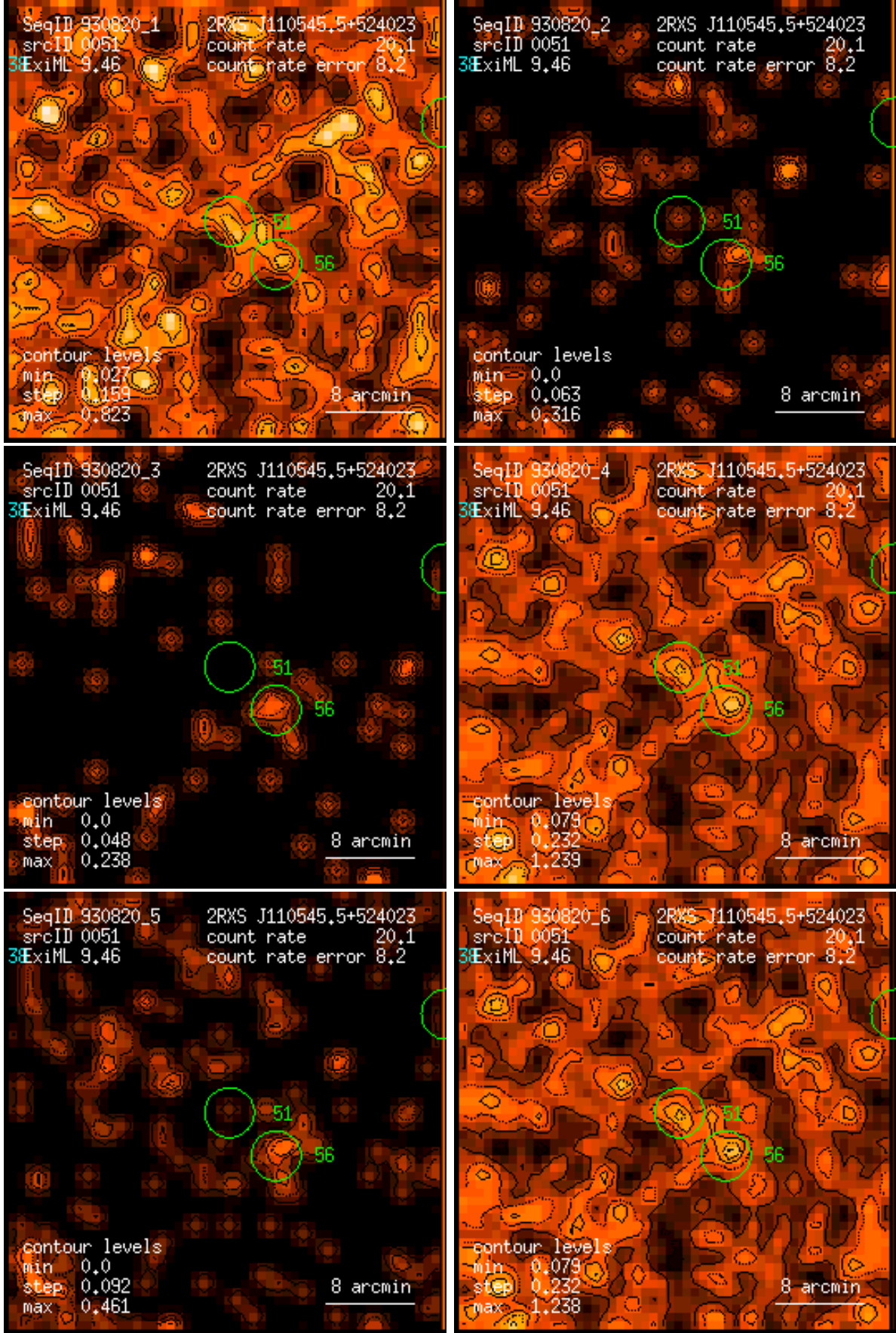
Figure 51: RASS 930820: detection 0051: band rate images, Gaussian filter: (1) PSPC channels 11 – 41, (2) 52 – 90, (3) 91 – 201, (4) 11 – 235, (5) 52 – 201, (6) 11 – 201. Broad band rates in counts/ks. Band rate contour levels in counts/ks/arcmin 2 .
