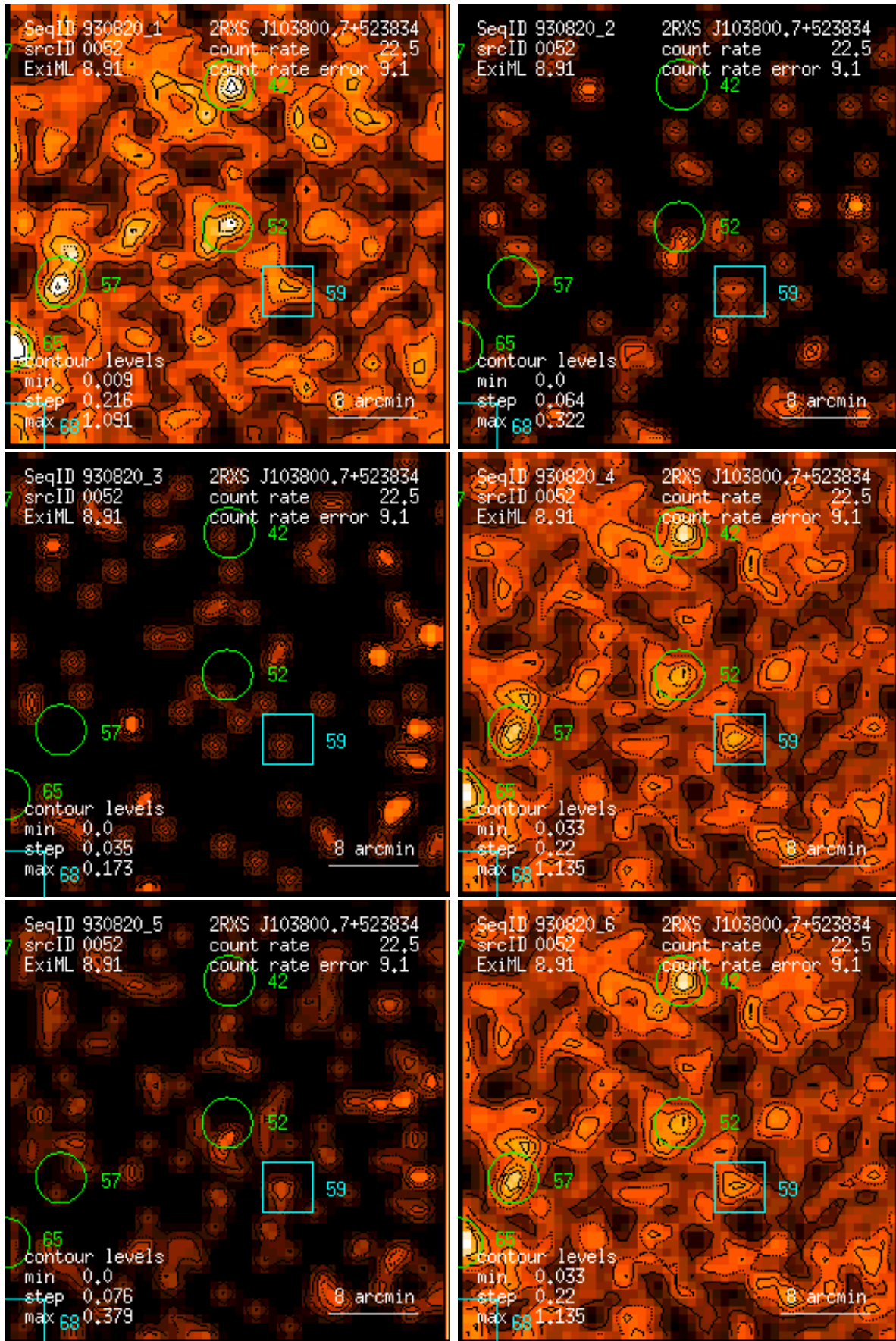
Figure 52: RASS 930820: detection 0052: band rate images, Gaussian filter: (1) PSPC channels 11 – 41, (2) 52 – 90, (3) 91 – 201, (4) 11 – 235, (5) 52 – 201, (6) 11 – 201. Broad band rates in counts/ks. Band rate contour levels in counts/ks/arcmin 2 .
