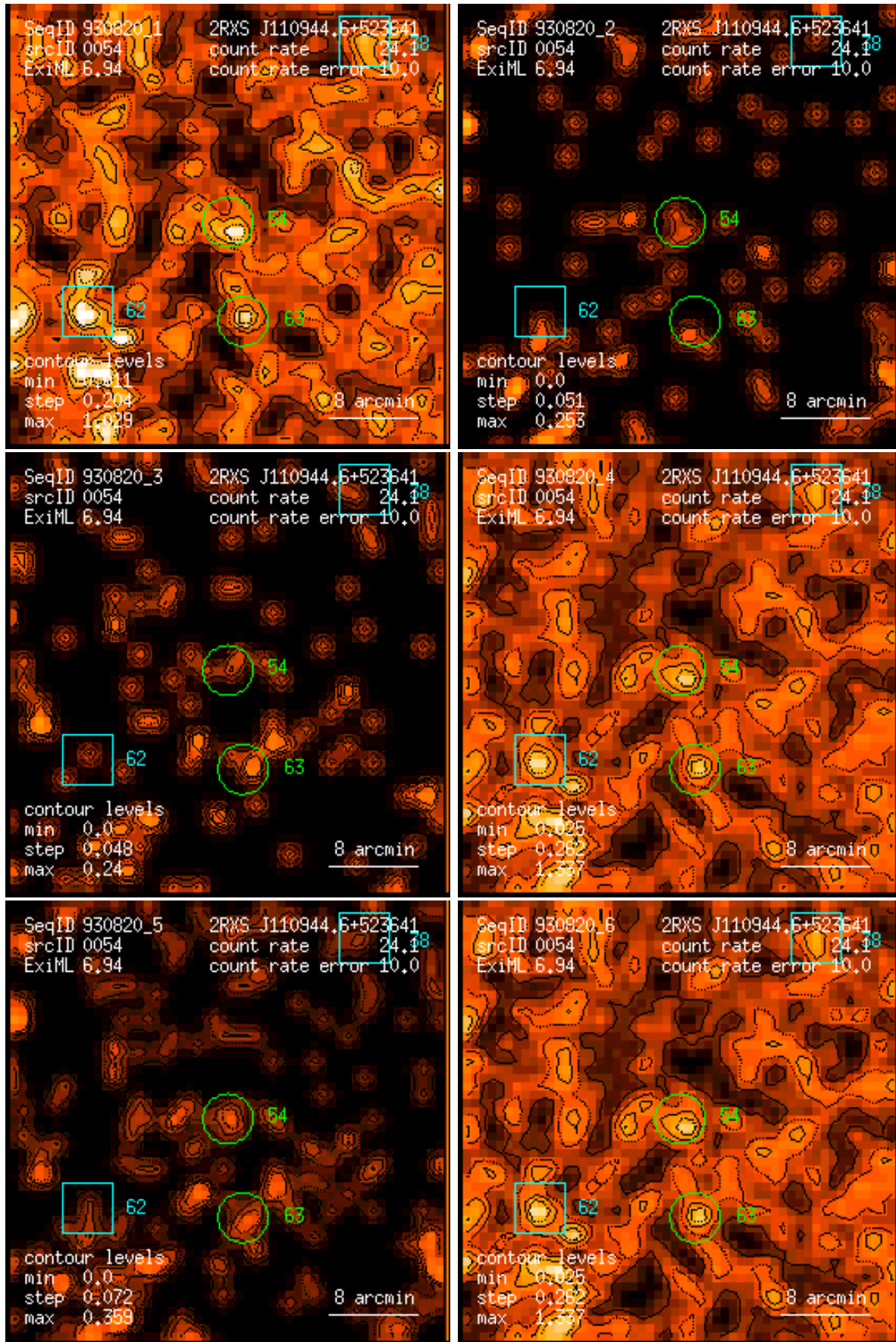
Figure 54: RASS 930820: detection 0054: band rate images, Gaussian filter: (1) PSPC channels 11 – 41, (2) 52 – 90, (3) 91 – 201, (4) 11 – 235, (5) 52 – 201, (6) 11 – 201. Broad band rates in counts/ks. Band rate contour levels in counts/ks/arcmin 2 .
