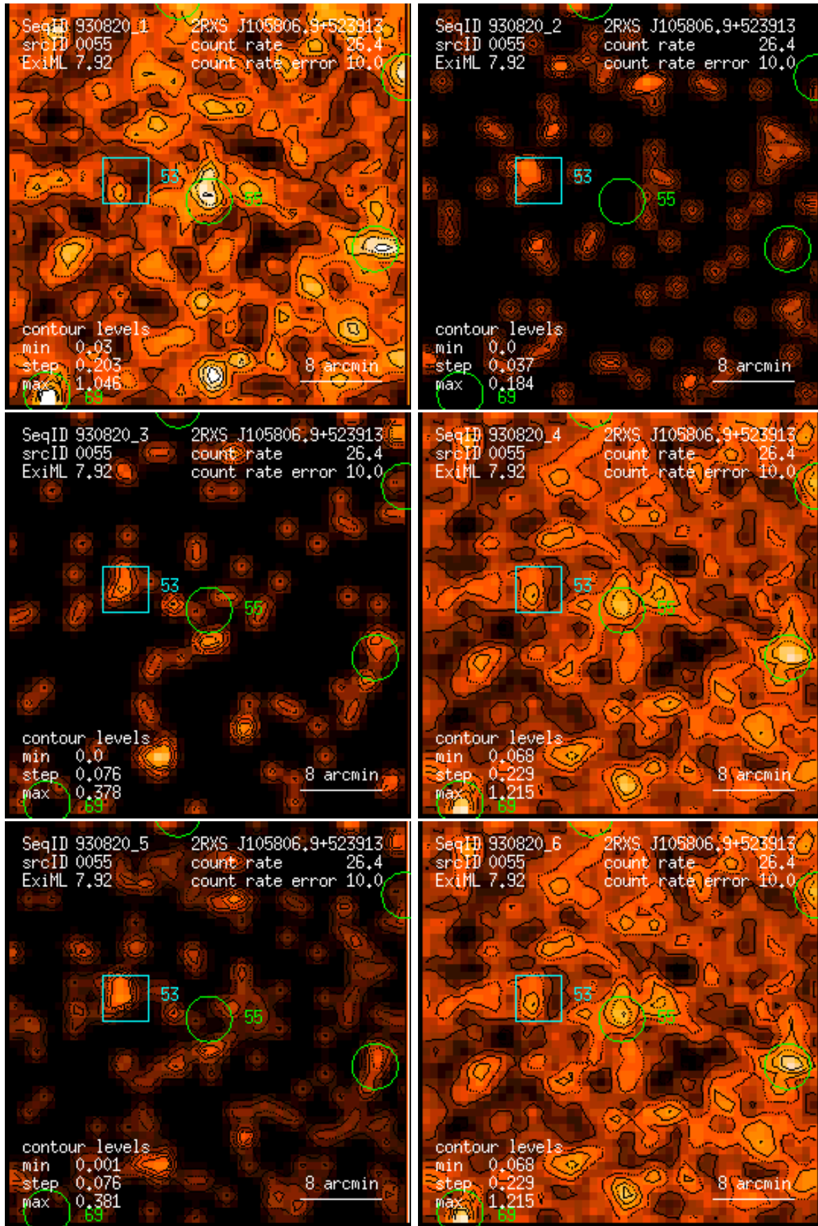
Figure 55: RASS 930820: detection 0055: band rate images, Gaussian filter: (1) PSPC channels 11 – 41, (2) 52 – 90, (3) 91 – 201, (4) 11 – 235, (5) 52 – 201, (6) 11 – 201. Broad band rates in counts/ks. Band rate contour levels in counts/ks/arcmin 2 .
