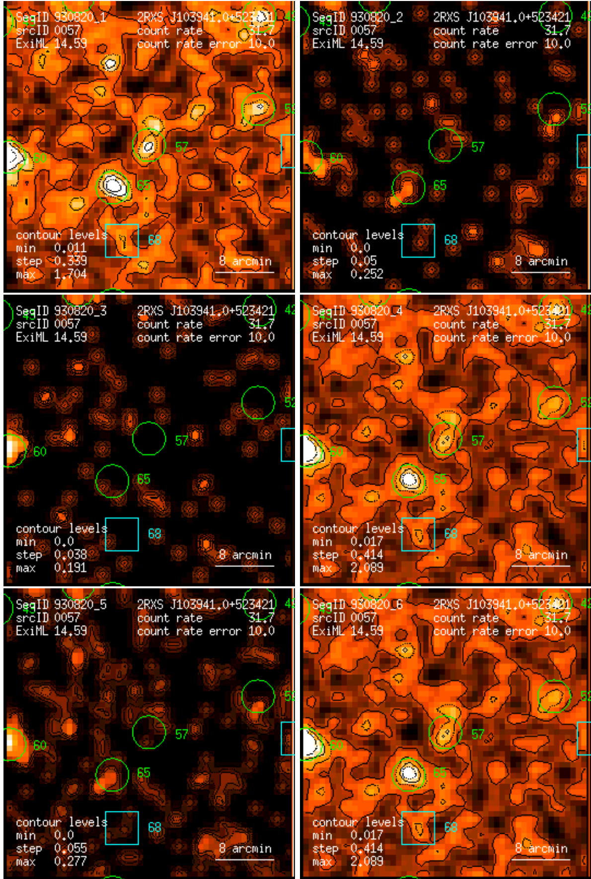
Figure 57: RASS 930820: detection 0057: band rate images, Gaussian filter: (1) PSPC channels 11 – 41, (2) 52 – 90, (3) 91 – 201, (4) 11 – 235, (5) 52 – 201, (6) 11 – 201. Broad band rates in counts/ks. Band rate contour levels in counts/ks/arcmin 2 .
