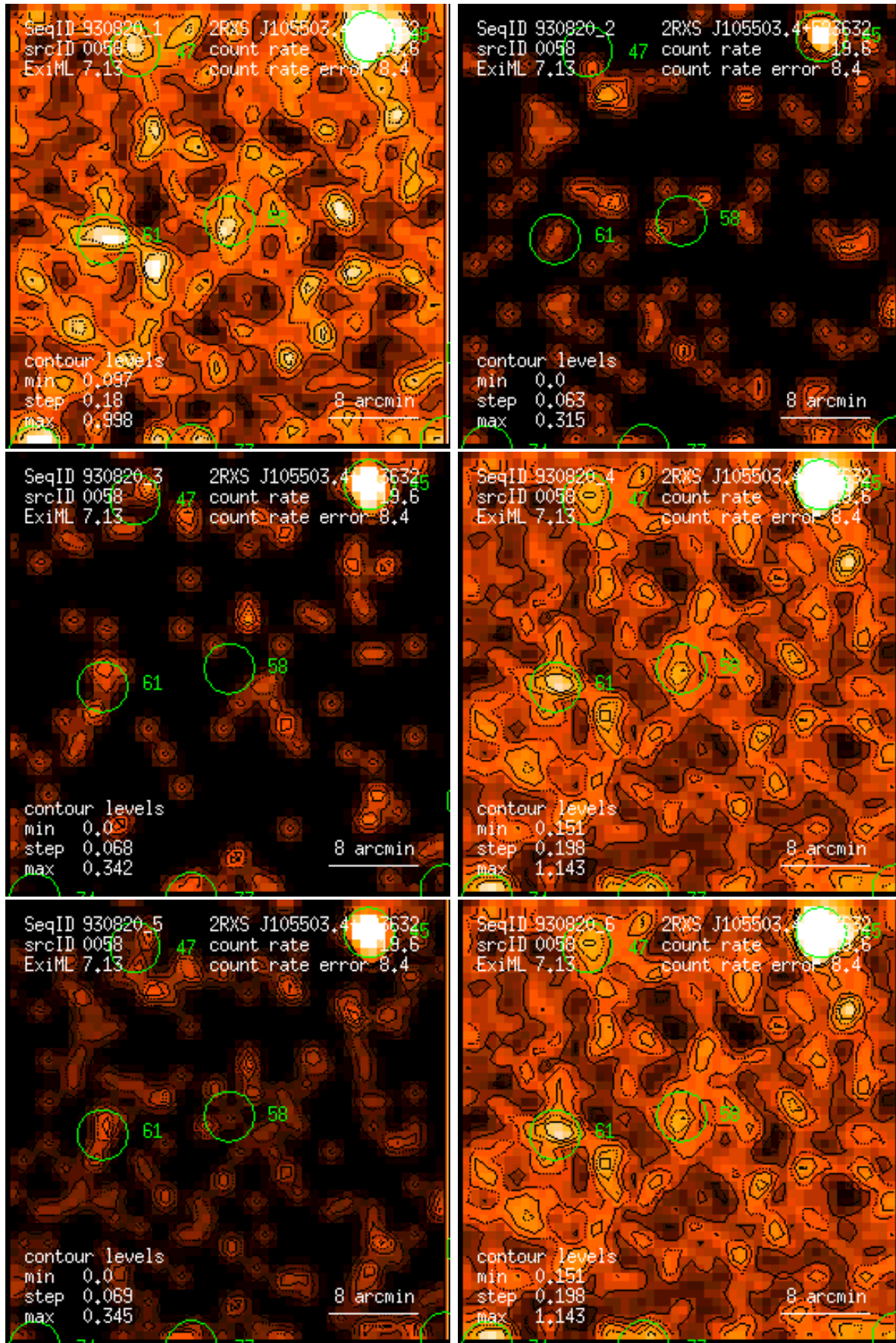
Figure 58: RASS 930820: detection 0058: band rate images, Gaussian filter: (1) PSPC channels 11 – 41, (2) 52 – 90, (3) 91 – 201, (4) 11 – 235, (5) 52 – 201, (6) 11 – 201. Broad band rates in counts/ks. Band rate contour levels in counts/ks/arcmin 2 .
