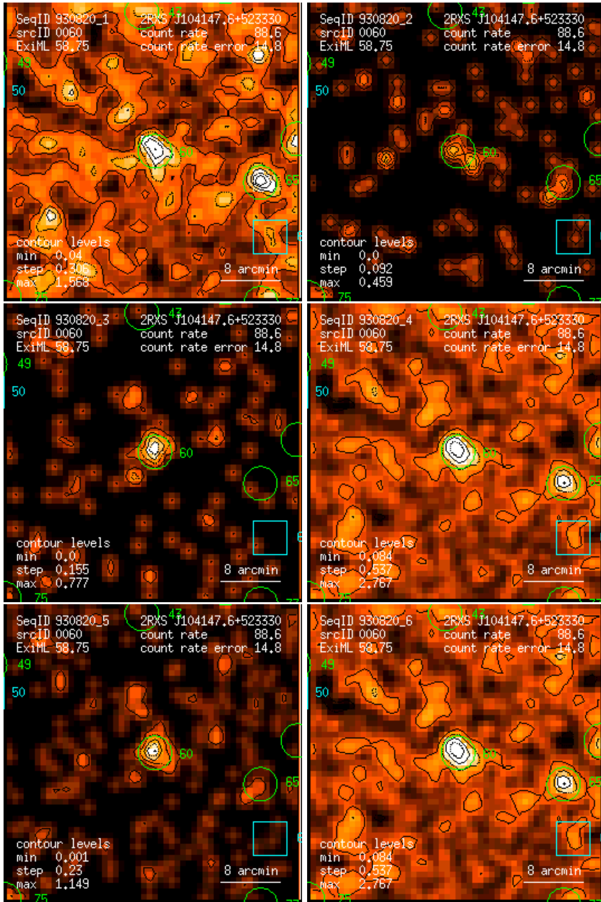
Figure 60: RASS 930820: detection 0060: band rate images, Gaussian filter: (1) PSPC channels 11 – 41, (2) 52 – 90, (3) 91 – 201, (4) 11 – 235, (5) 52 – 201, (6) 11 – 201. Broad band rates in counts/ks. Band rate contour levels in counts/ks/arcmin 2 .
