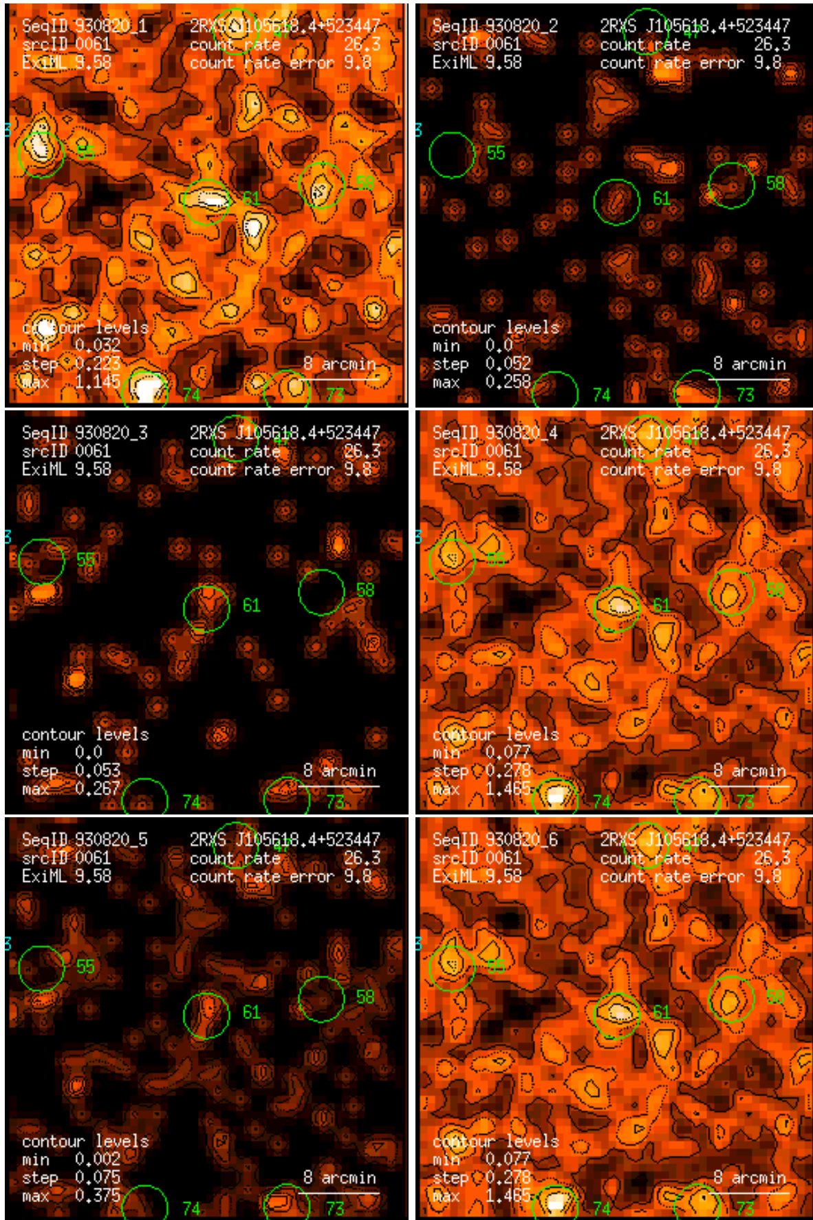
Figure 61: RASS 930820: detection 0061: band rate images, Gaussian filter: (1) PSPC channels 11 – 41, (2) 52 – 90, (3) 91 – 201, (4) 11 – 235, (5) 52 – 201, (6) 11 – 201. Broad band rates in counts/ks. Band rate contour levels in counts/ks/arcmin 2 .
