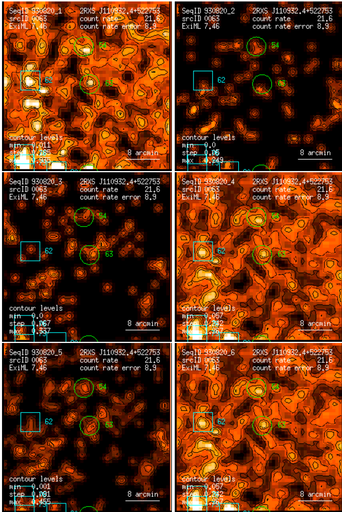
Figure 63: RASS 930820: detection 0063: band rate images, Gaussian filter: (1) PSPC channels 11 – 41, (2) 52 – 90, (3) 91 – 201, (4) 11 – 235, (5) 52 – 201, (6) 11 – 201. Broad band rates in counts/ks. Band rate contour levels in counts/ks/arcmin 2 .
