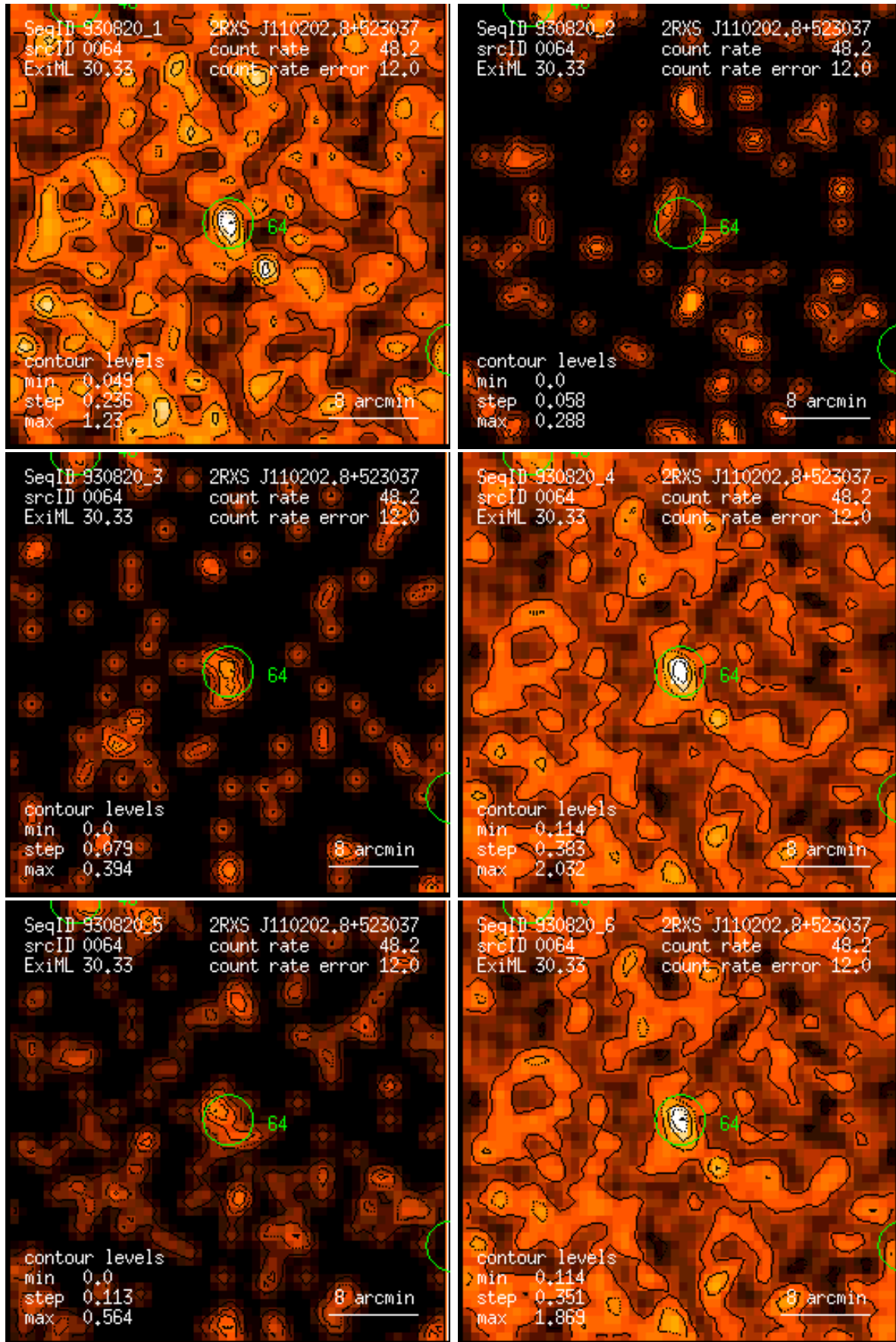
Figure 64: RASS 930820: detection 0064: band rate images, Gaussian filter: (1) PSPC channels 11 – 41, (2) 52 – 90, (3) 91 – 201, (4) 11 – 235, (5) 52 – 201, (6) 11 – 201. Broad band rates in counts/ks. Band rate contour levels in counts/ks/arcmin 2 .
