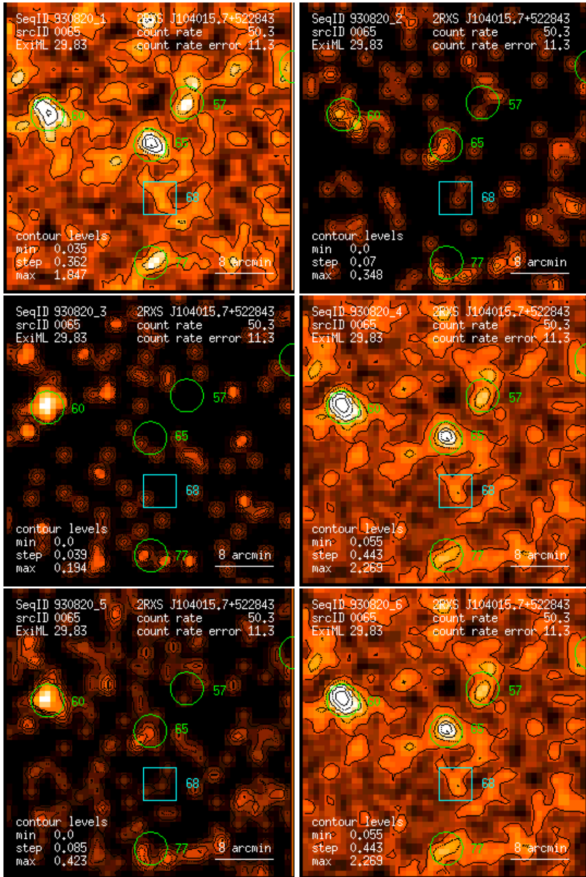
Figure 65: RASS 930820: detection 0065: band rate images, Gaussian filter: (1) PSPC channels 11 – 41, (2) 52 – 90, (3) 91 – 201, (4) 11 – 235, (5) 52 – 201, (6) 11 – 201. Broad band rates in counts/ks. Band rate contour levels in counts/ks/arcmin 2 .
