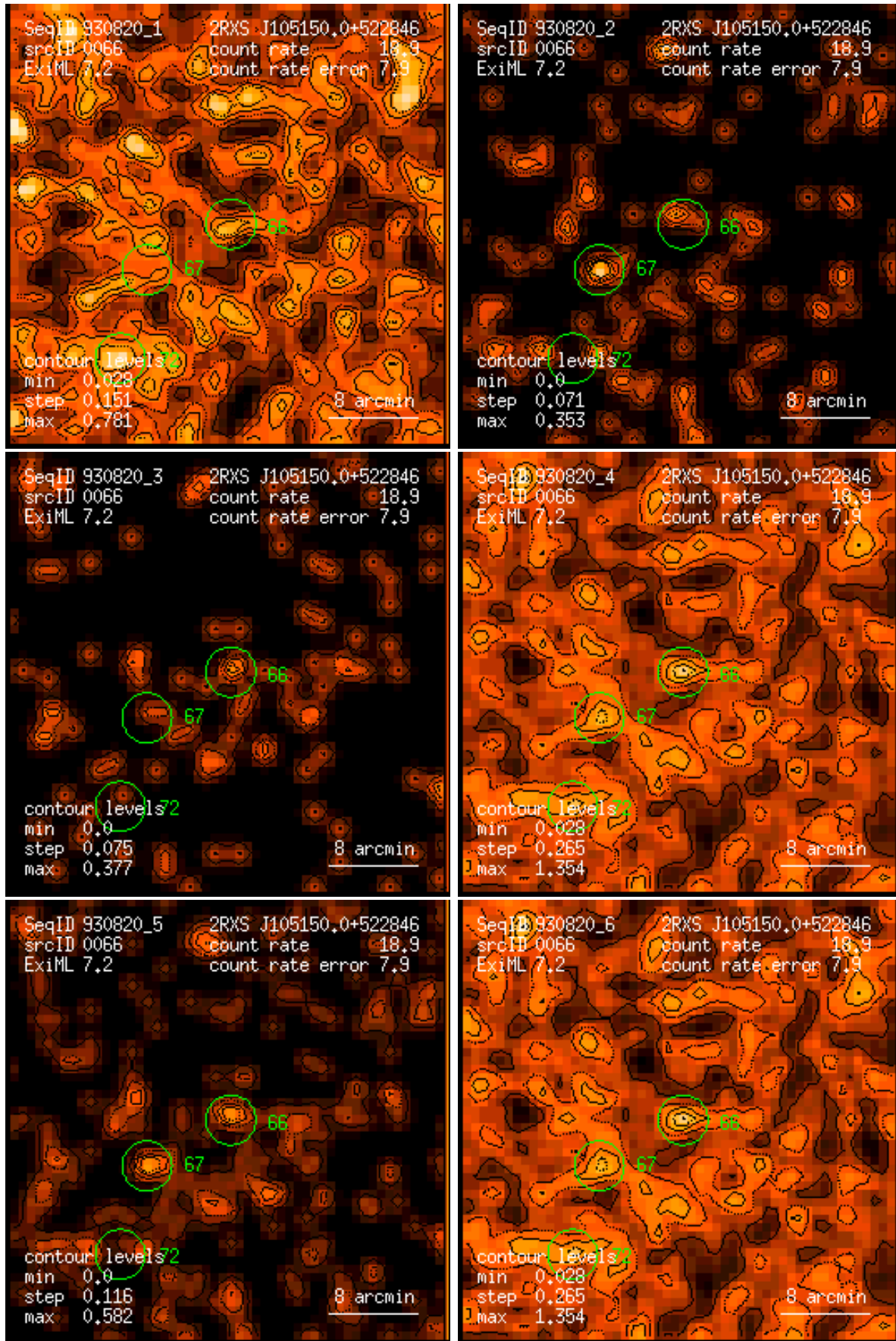
Figure 66: RASS 930820: detection 0066: band rate images, Gaussian filter: (1) PSPC channels 11 – 41, (2) 52 – 90, (3) 91 – 201, (4) 11 – 235, (5) 52 – 201, (6) 11 – 201. Broad band rates in counts/ks. Band rate contour levels in counts/ks/arcmin 2 .
