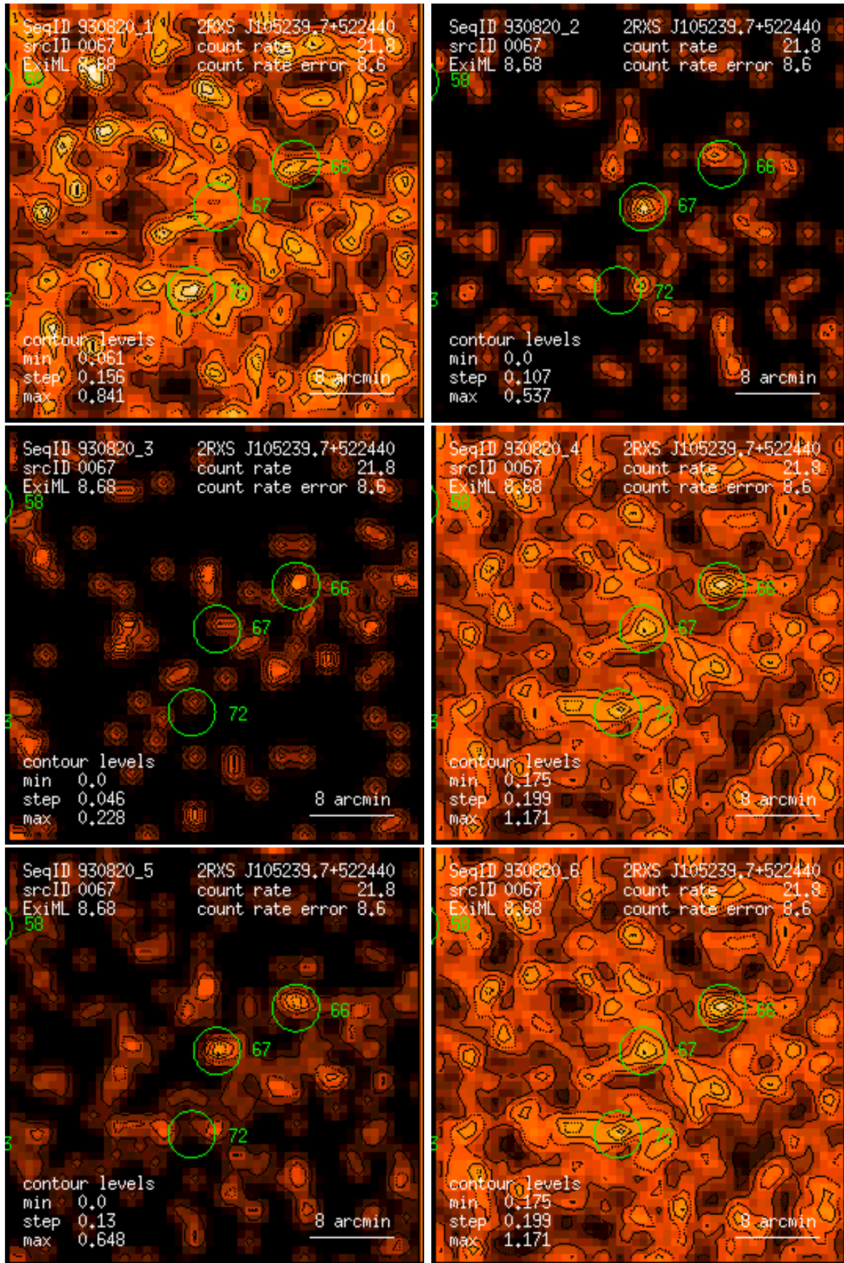
Figure 67: RASS 930820: detection 0067: band rate images, Gaussian filter: (1) PSPC channels 11 – 41, (2) 52 – 90, (3) 91 – 201, (4) 11 – 235, (5) 52 – 201, (6) 11 – 201. Broad band rates in counts/ks. Band rate contour levels in counts/ks/arcmin 2 .
