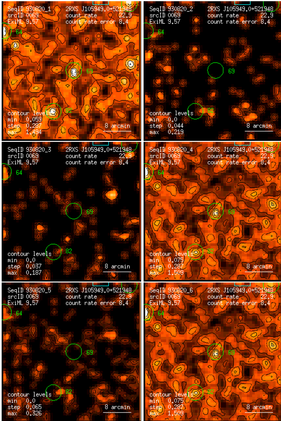
Figure 69: RASS 930820: detection 0069: band rate images, Gaussian filter: (1) PSPC channels 11 – 41, (2) 52 – 90, (3) 91 – 201, (4) 11 – 235, (5) 52 – 201, (6) 11 – 201. Broad band rates in counts/ks. Band rate contour levels in counts/ks/arcmin 2 .
