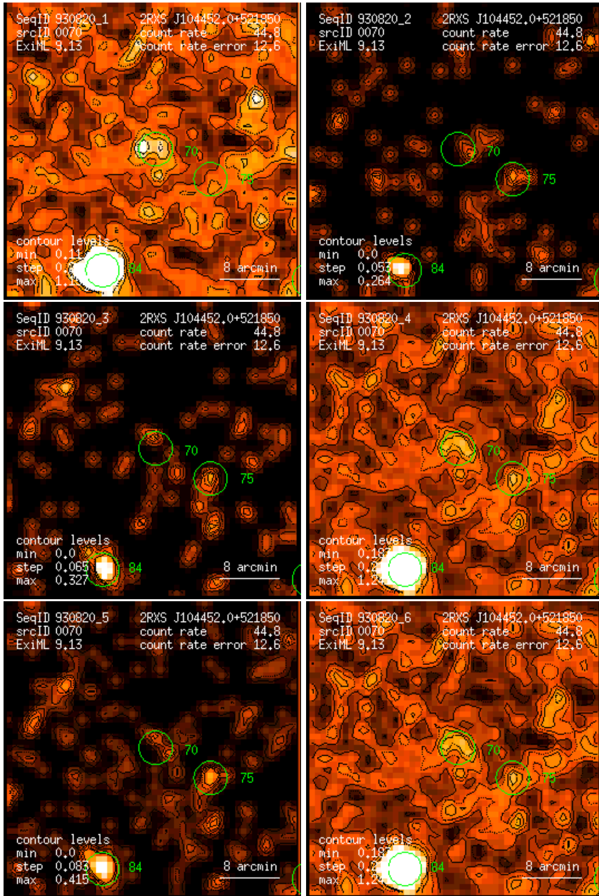
Figure 70: RASS 930820: detection 0070: band rate images, Gaussian filter: (1) PSPC channels 11 – 41, (2) 52 – 90, (3) 91 – 201, (4) 11 – 235, (5) 52 – 201, (6) 11 – 201. Broad band rates in counts/ks. Band rate contour levels in counts/ks/arcmin 2 .
