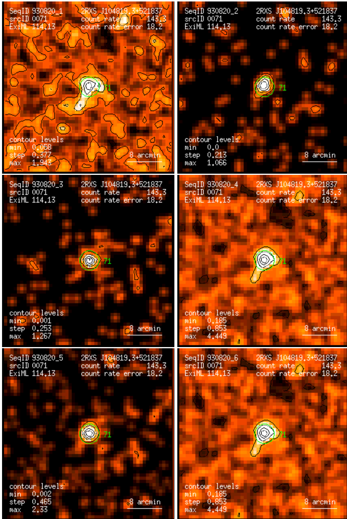
Figure 71: RASS 930820: detection 0071: band rate images, Gaussian filter: (1) PSPC channels 11 – 41, (2) 52 – 90, (3) 91 – 201, (4) 11 – 235, (5) 52 – 201, (6) 11 – 201. Broad band rates in counts/ks. Band rate contour levels in counts/ks/arcmin 2 .
