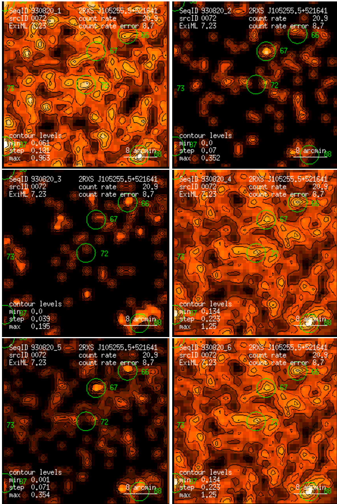
Figure 72: RASS 930820: detection 0072: band rate images, Gaussian filter: (1) PSPC channels 11 – 41, (2) 52 – 90, (3) 91 – 201, (4) 11 – 235, (5) 52 – 201, (6) 11 – 201. Broad band rates in counts/ks. Band rate contour levels in counts/ks/arcmin 2 .
