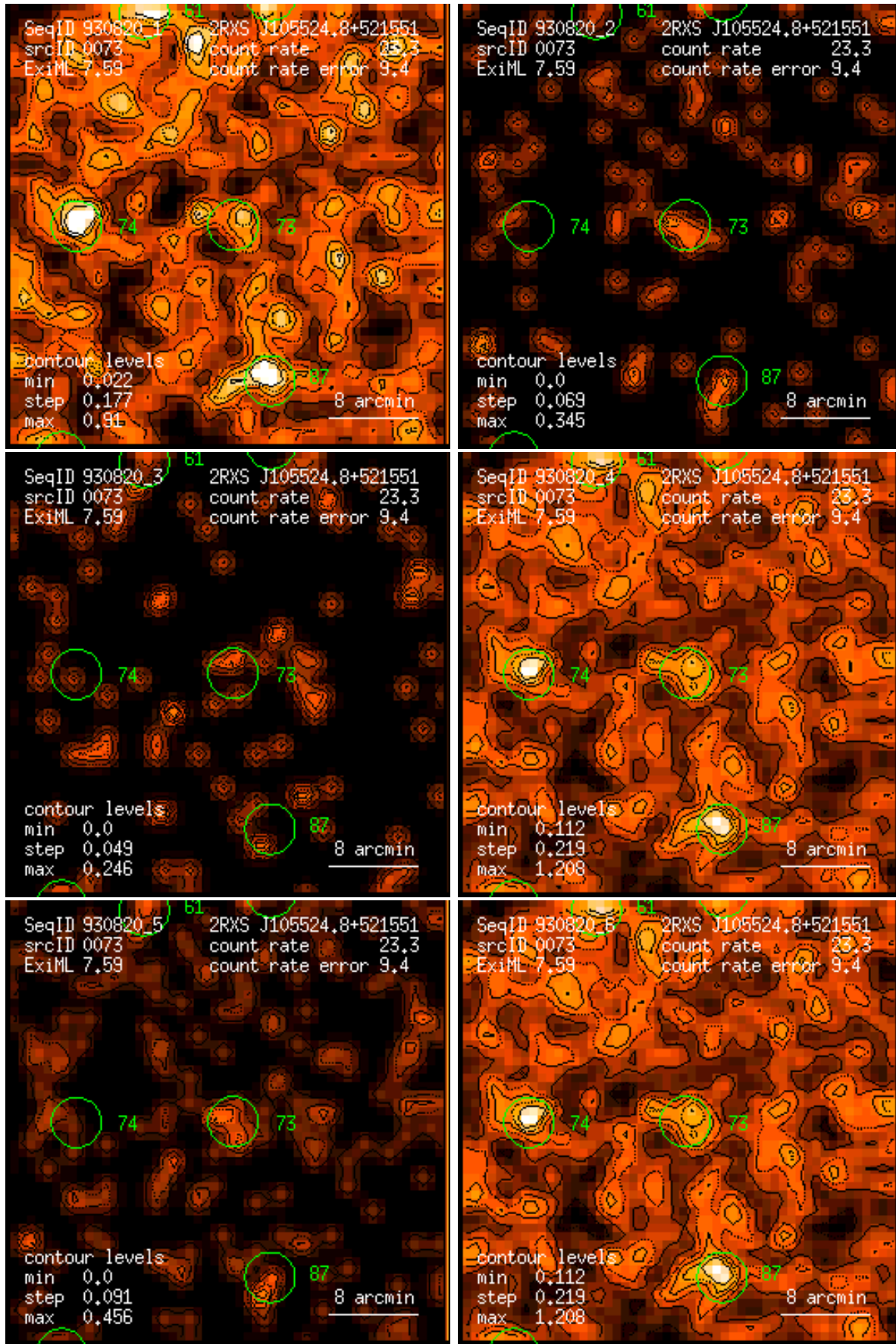
Figure 73: RASS 930820: detection 0073: band rate images, Gaussian filter: (1) PSPC channels 11 – 41, (2) 52 – 90, (3) 91 – 201, (4) 11 – 235, (5) 52 – 201, (6) 11 – 201. Broad band rates in counts/ks. Band rate contour levels in counts/ks/arcmin 2 .
